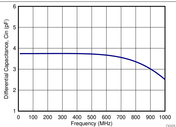
Figure 174. Differential Input Capacitance (C IN )
