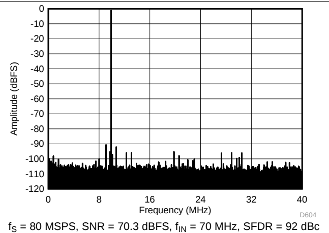
Figure 70. FFT for 70-MHz Input Signal (Dither Off)
