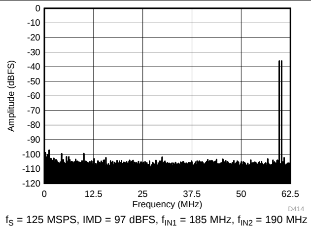
Figure 47. FFT for Two-Tone Input Signal ( -36\text{ dBFS} at 185\text{ MHz} and 190\text{ MHz} )
