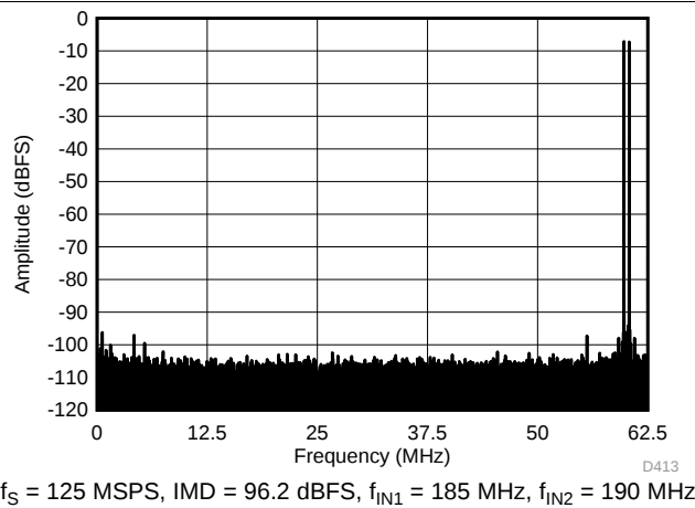
Figure 46. FFT for Two-Tone Input Signal ( -7\text{ dBFS} at 185\text{ MHz} and 190\text{ MHz} )
