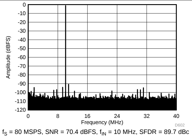
Figure 68. FFT for 10-MHz Input Signal (Dither Off)
