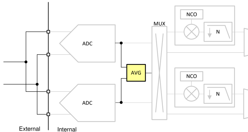
图 8-45. Digital Channel Averaging Diagram
