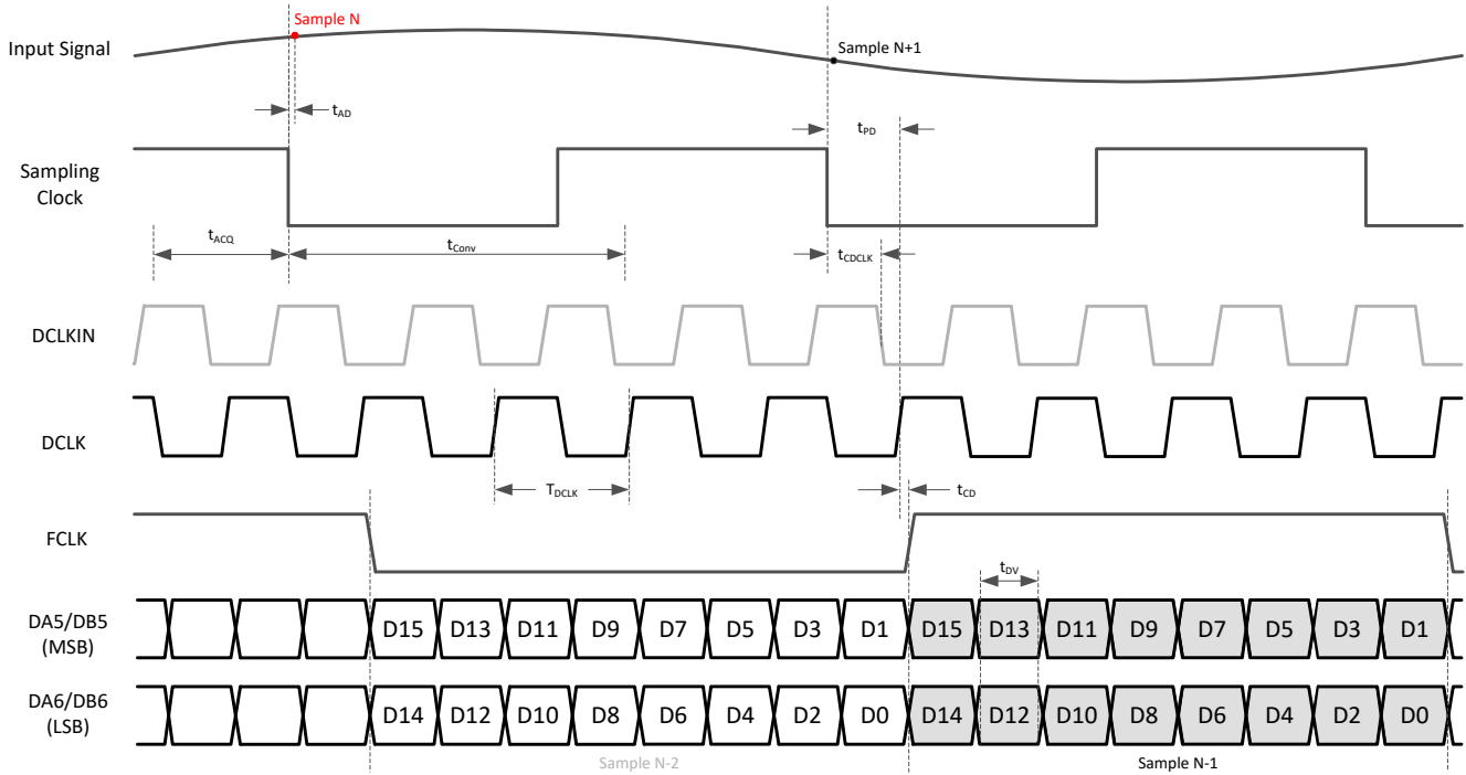
图 7-1. Timing diagram: 2-wire SCAMOS (changed from 18-bit to 16-bit output after power up)
