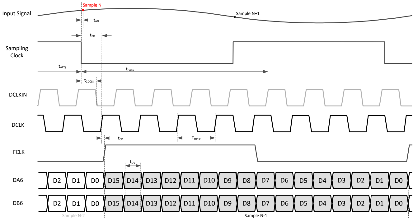
图 7-2. Timing diagram: 1-wire SCAMOS (changed from 18-bit to 16-bit output after power up)
