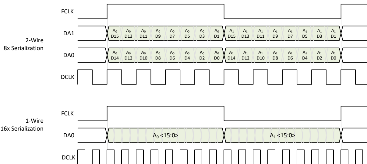
图 8-38. Output Data Format in Real Decimation
