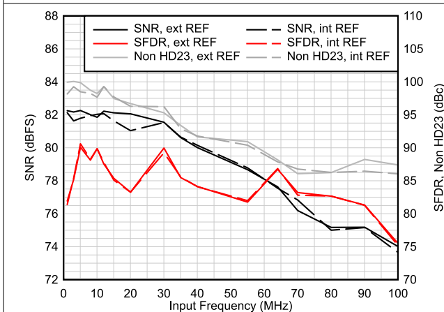
图 6-11. AC Performance vs Input Frequency
