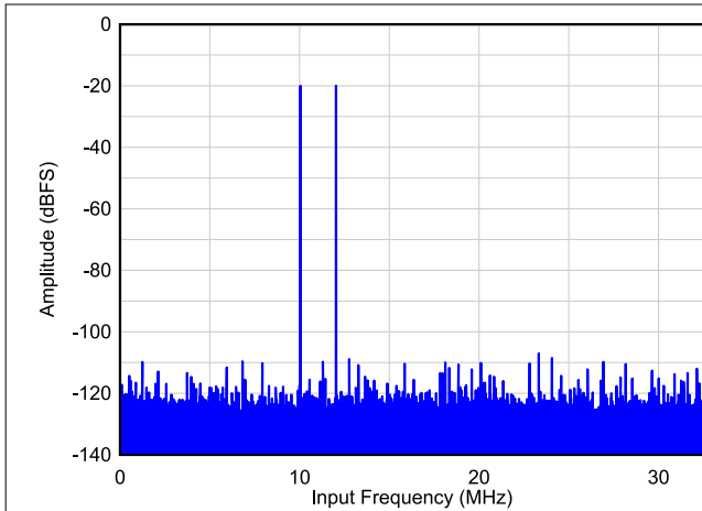
A_{IN} = -20\text{ dBFS/tone} , IMD3 = 98\text{ dBc}
