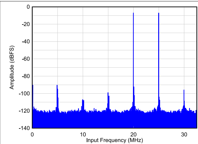
A_{IN} = -7\text{ dBFS/tone} , IMD3 = 89\text{ dBc}
