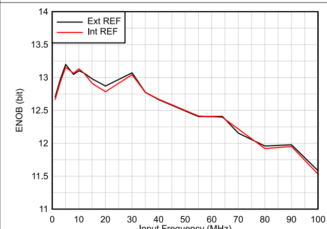
图 6-12. ENOB vs Input Frequency
