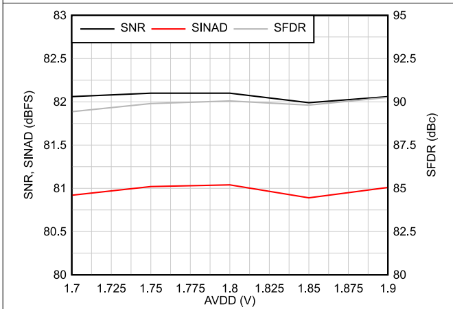
图 6-17. AC Performance vs AVDD
