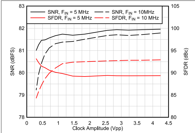
图 6-15. AC Performance vs Clock Amplitude
