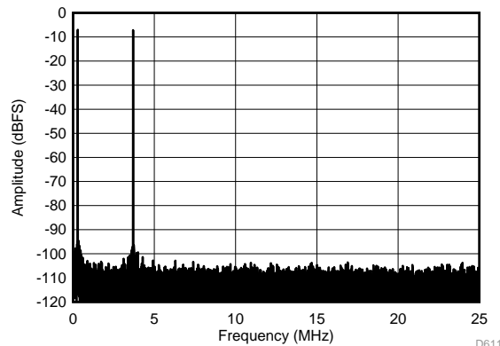
f_{IN1} = 46\text{ MHz} , f_{IN2} = 50\text{ MHz} , IMD3 = 102 dBFS, each tone at -7\text{ dBFS}
