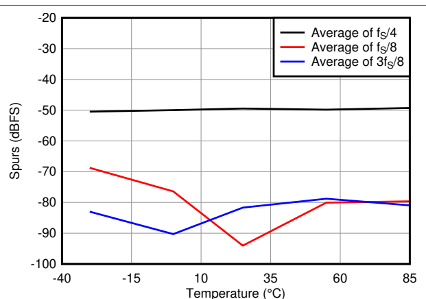
图 9-8. Offset Corrector Block Disabled
