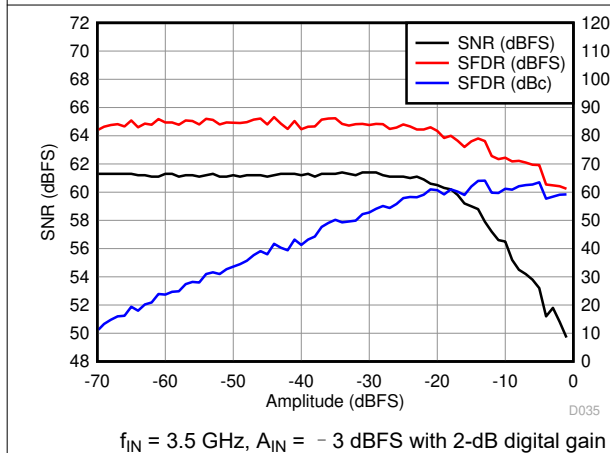
图 6-59. Performance vs. Amplitude
