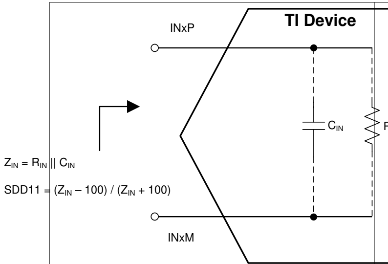
Copyright © 2016, Texas Instruments Incorporated 图 8-1. Equivalent Input Impedance
