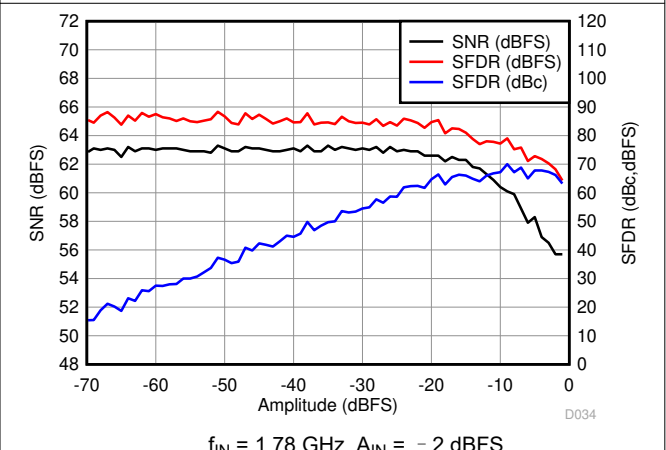
图 6-58. Performance vs. Amplitude
