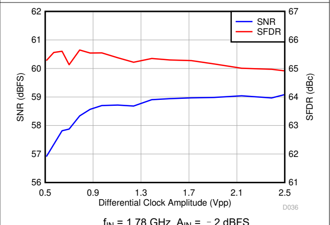
图 6-60. Performance vs. Clock Amplitude
