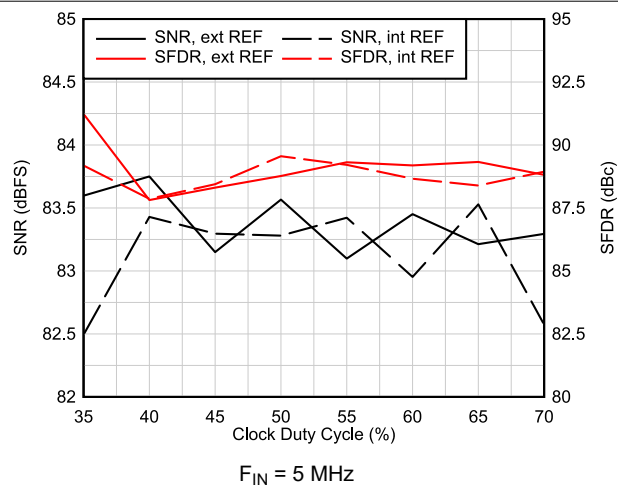
Figure 6-19. AC Performance vs Clock Duty Cycle
