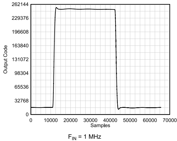
Figure 6-23. Pulse Response
