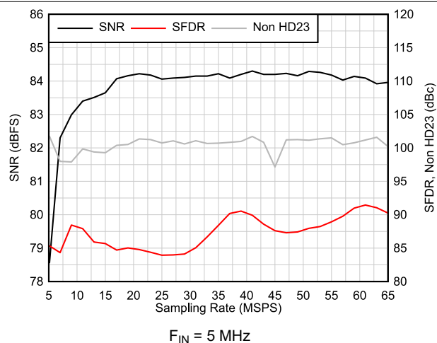
Figure 6-14. AC Performance vs Sampling Rate
