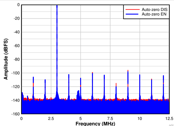
Figure 8-8. FFT at 25 MSPS with input frequency of 3 MHz (auto-zero feature enable vs disable, 4M point FFT)
