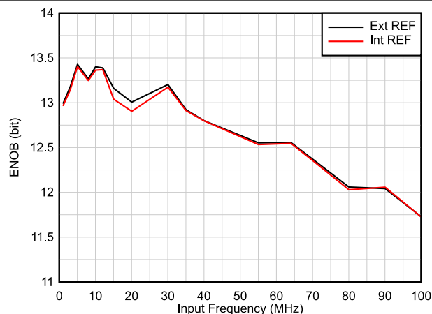
Figure 6-12. ENOB vs Input Frequency
