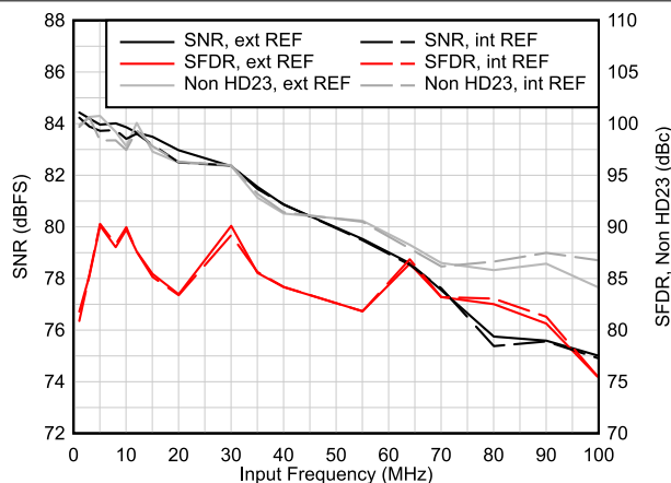
Figure 6-11. AC Performance vs Input Frequency
