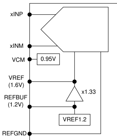
Figure 8-15. Different voltage reference options for ADC358x
