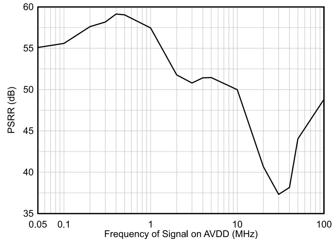
Figure 11-1. Power supply rejection ratio (PSRR) vs frequency
