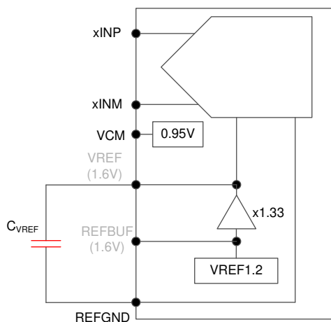
Figure 8-16. Internal reference
