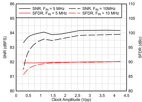
Figure 8-12. AC Performance vs Clock Amplitude (Differential Clock Input)
