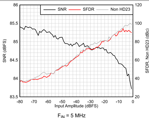
Figure 6-13. AC Performance vs Input Amplitude
