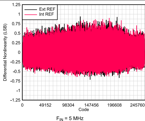
Figure 6-21. DNL vs Code
