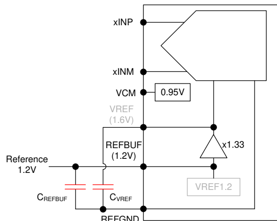
Figure 8-18. External 1.2V reference using internal reference buffer
