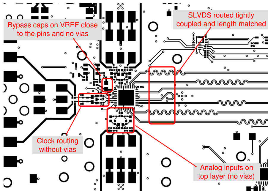
Figure 12-1. Layout example: top layer of ADC358x/368x EVM
