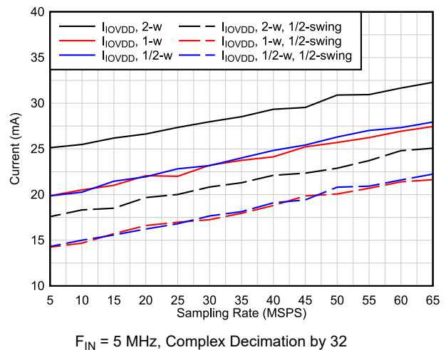
Figure 6-26. I_{IOVDD} Current vs Output Interface
