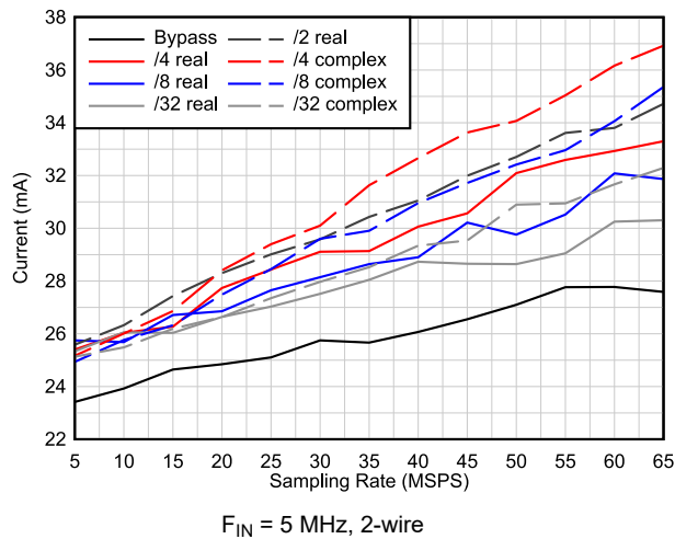
Figure 6-25. I_{IOVDD} Current vs Decimation
