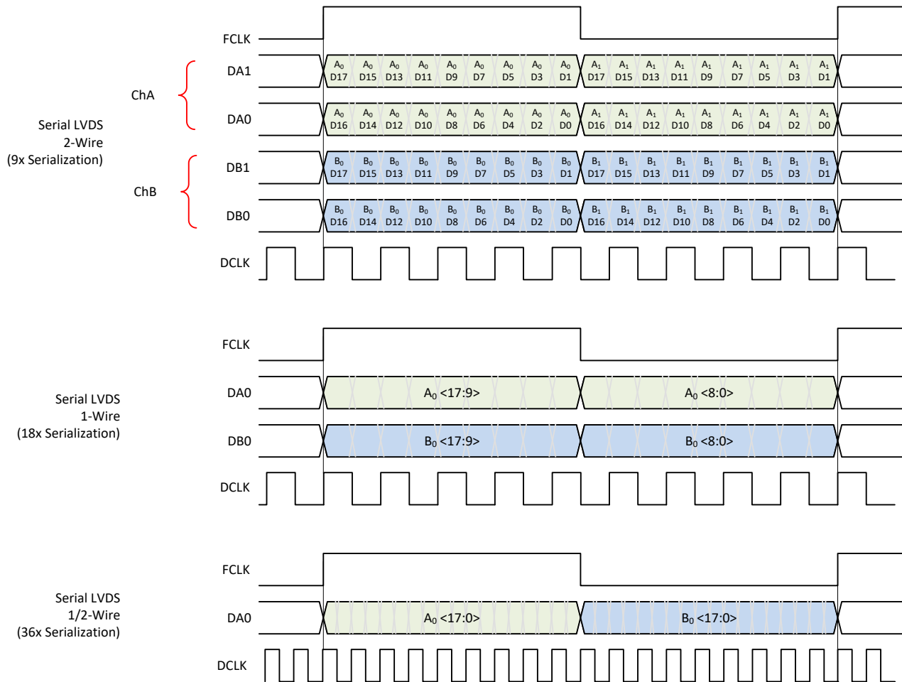
Figure 8-38. Output Data Format in Real Decimation (18-bit Output Resolution)
