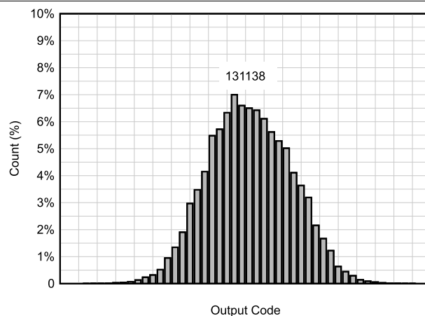
Figure 6-22. DC Histogram
