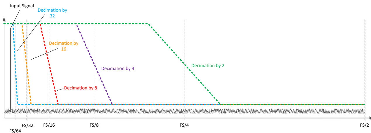
Figure 8-23. Real decimation illustration
