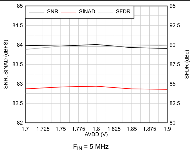
Figure 6-17. AC Performance vs AVDD
