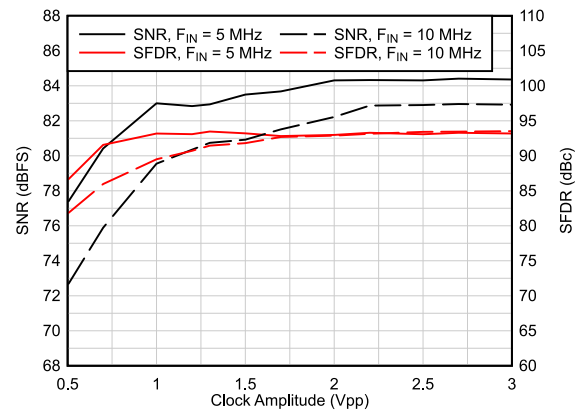
Figure 8-13. AC Performance vs Clock Amplitude (Single Ended Clock Input)
