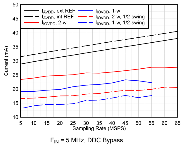
Figure 6-24. Current vs Sampling Rate
