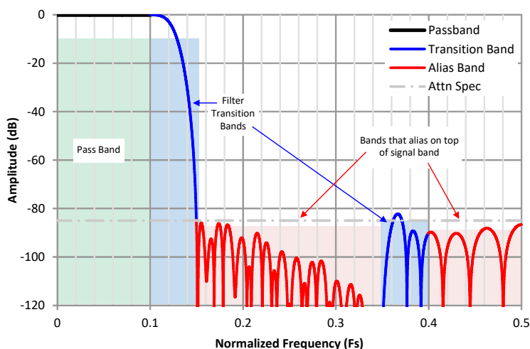
Figure 8-25. Interpretation of the Decimation Filter Plots
