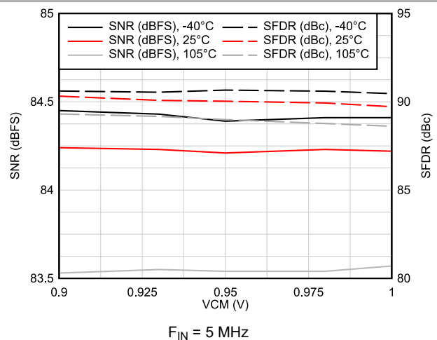
Figure 6-18. AC Performance vs VCM vs Temperature
