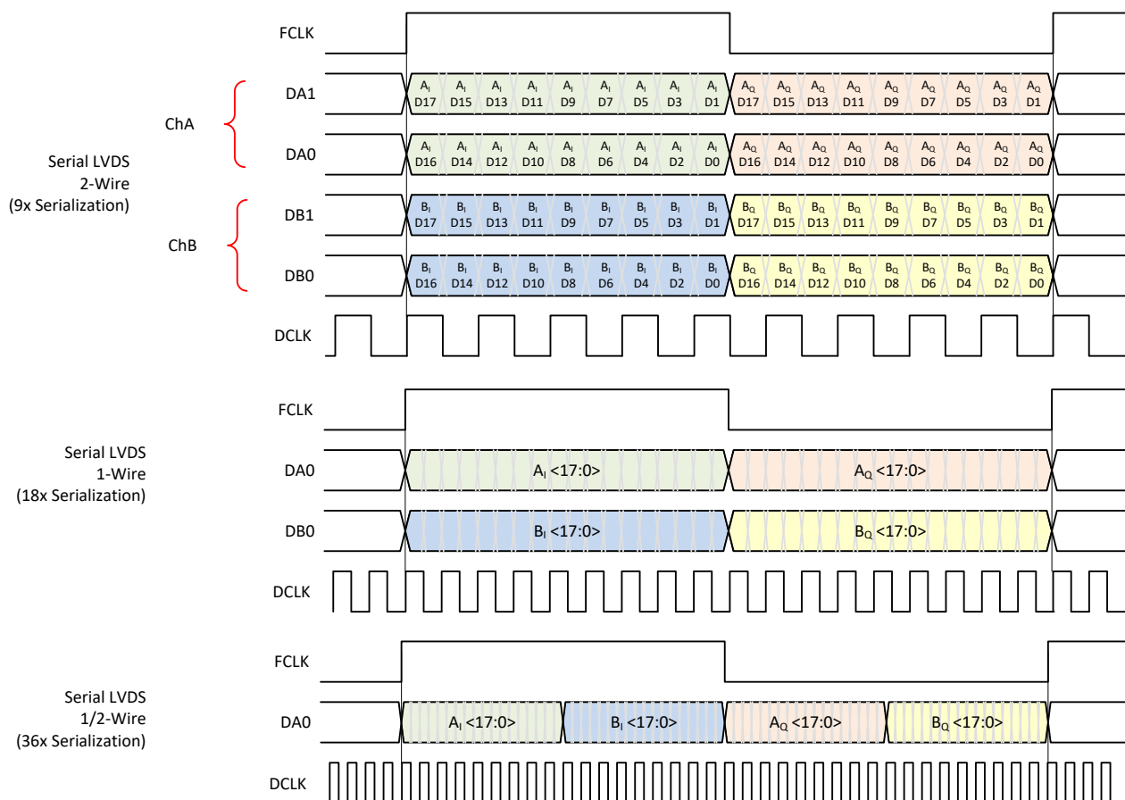
Figure 8-37. Output Data Format in Complex Decimation (18-bit Output Resolution)
