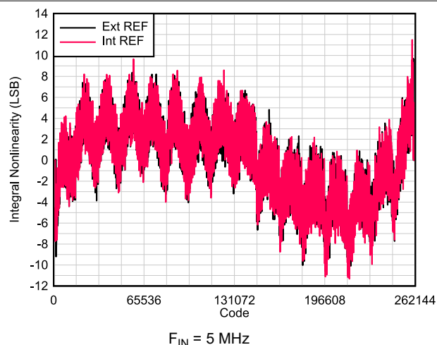
Figure 6-20. INL vs Code
