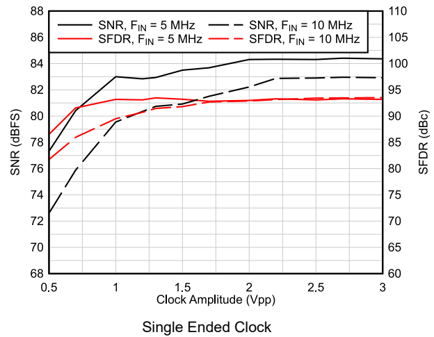
Figure 6-16. AC Performance vs Clock Amplitude
