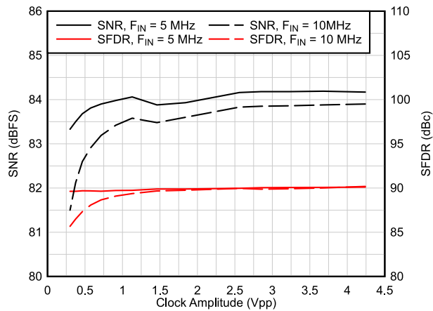
Figure 6-15. AC Performance vs Clock Amplitude
