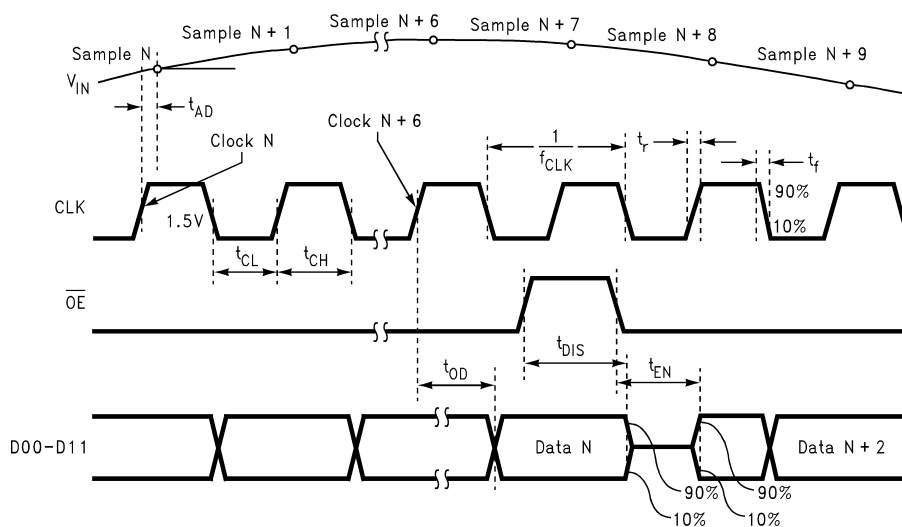
Figure 3. Output Timing
