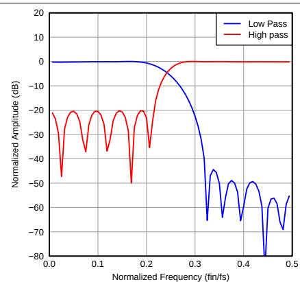
图 31. Filter Response, Decimate by 2
