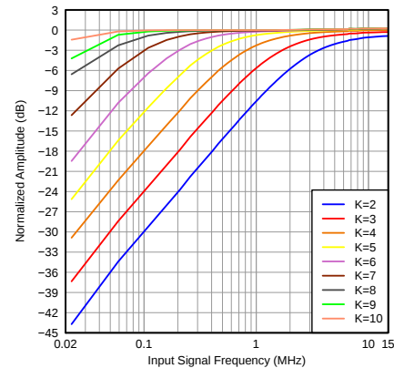
图 35. Digital High-Pass Filter Response
