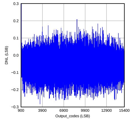
图 27. Differential Non-Linearity
