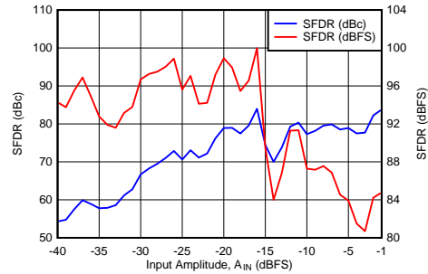
32-input mode, 14-bit resolution, f_{SAMP} = 32.5 MSPS 图 23. Spurious-Free Dynamic Range vs A_{IN}
