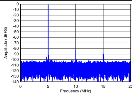
f_{IN} = 5 MHz, f_C = 80 MSPS, SNR = 69.9 dBFS, SFDR = 82.6 dBc, HD2 = -82.6 dBc, HD3 = -88.9 dBc
