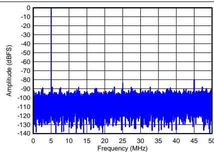
f_{IN} = 5 MHz, f_C = 100 MSPS, SNR = 61.6 dBFS, SFDR = 78.7 dBc, HD2 = -97.6 dBc, HD3 = -92.2 dBc
