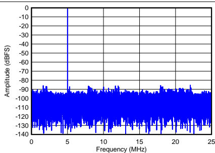
f_{IN} = 5 MHz, f_C = 100 MSPS, SNR = 61.5 dBFS, SFDR = 81.9 dBc, HD2 = -86.5 dBc, HD3 = -93.9 dBc
