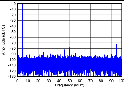
f_{IN} = 5 MHz, f_C = 100 MSPS, SNR = 61.3 dBFS, SFDR = 70.8 dBc, HD2 = -94.2 dBc, HD3 = -80.1 dBc
