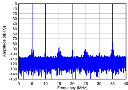
f_{IN} = 5 MHz, f_C = 80 MSPS, SNR = 70.2 dBFS, SFDR = 75.4 dBc, HD2 = -109.8 dBc, HD3 = -86.1 dBc
