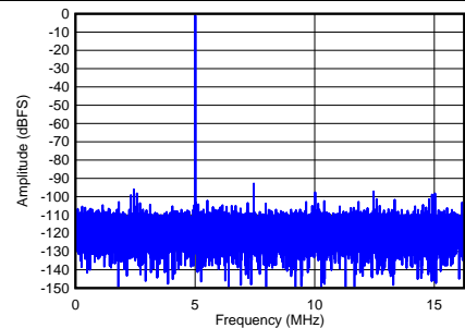
f_{IN} = 5 MHz, f_C = 65 MSPS, SNR = 73.7 dBFS, SFDR = 91.8 dBc, HD2 = -96.6 dBc, HD3 = -97.2 dBc
