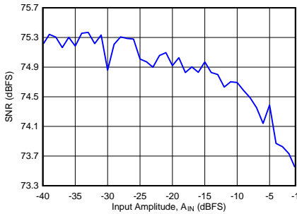
16-input mode, 14-bit resolution, f_{SAMP} = 65 MSPS 图 22. Signal-to-Noise Ratio vs A_{IN}
