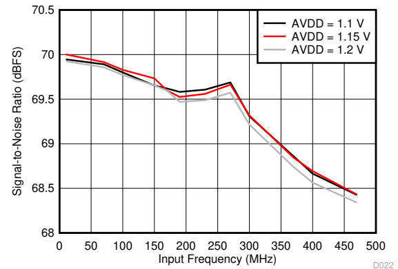
图 6-23. SNR vs Input Frequency and AVDD Supply
