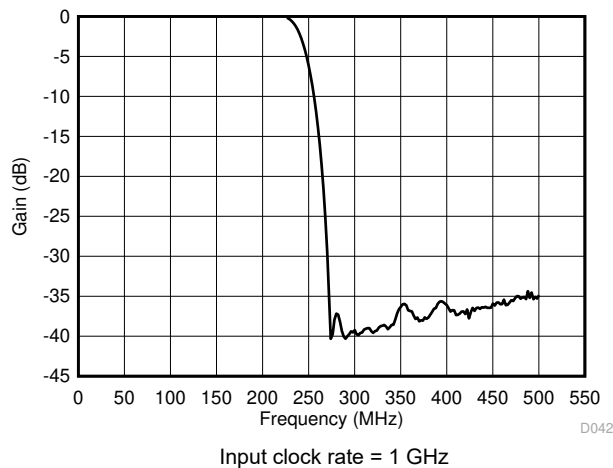
图 7-5. Decimation Filter Response vs Frequency
