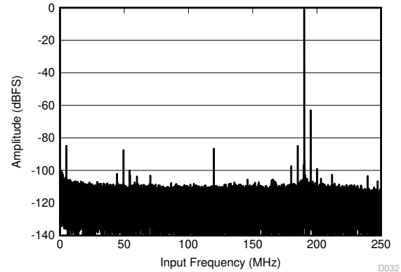
图 6-33. Common-Mode Rejection Ratio FFT
