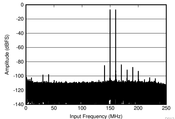
图 6-11. FFT for Two-Tone Input Signal
