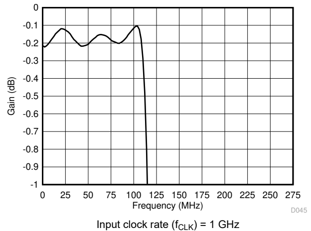
图 7-8. Decimation Filter Pass-Band Ripple vs Frequency
