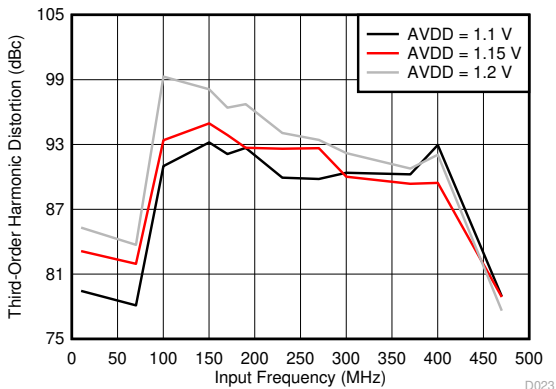
图 6-24. HD3 vs Input Frequency and AVDD Supply
