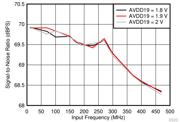
图 6-21. SNR vs Input Frequency and AVDD19 Supply
