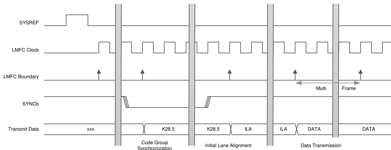
图 7-23. ILA Sequence
