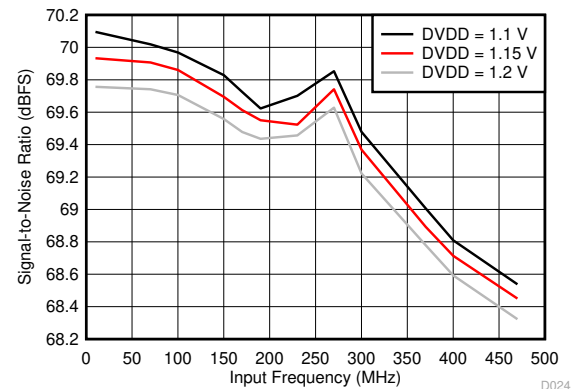
图 6-25. SNR vs Input Frequency and DVDD Supply
