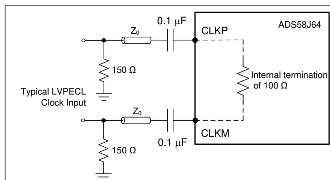
图 7-2. LVPECL Clock Driving Circuit
