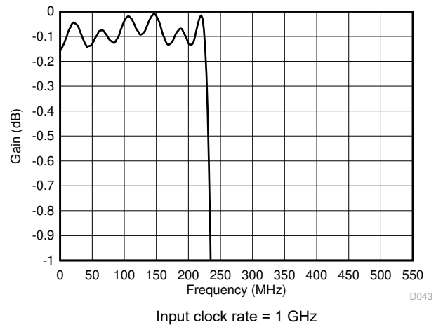
图 7-6. Decimation Filter Pass-Band Ripple vs Frequency
