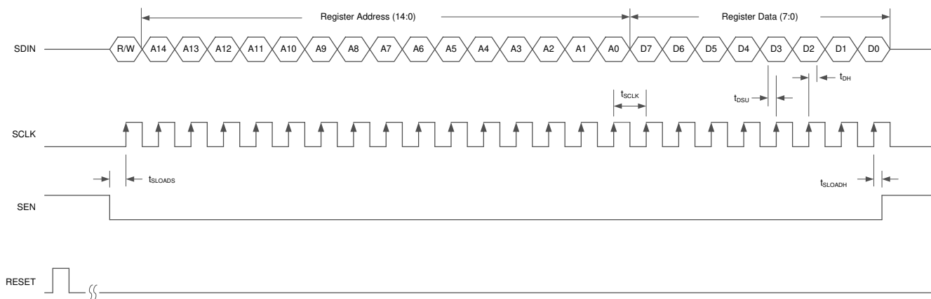
图 7-30. Serial Interface Write Timing Diagram
