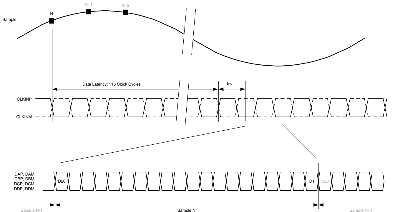
图 6-1. Latency Timing Diagram in Burst Mode
