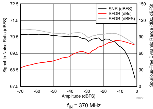
图 6-28. Performance vs Input Signal Amplitude
