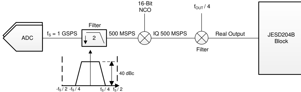
图 7-12. Operating Mode 3
