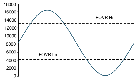
图 7-20. FOVR High and FOVR Low Thresholds
