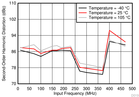
图 6-20. HD2 vs Input Frequency and Temperature
