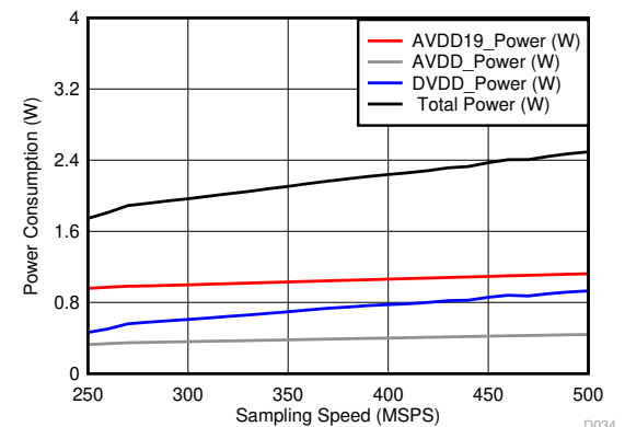
图 6-35. Power Consumption vs Input Clock Rate
