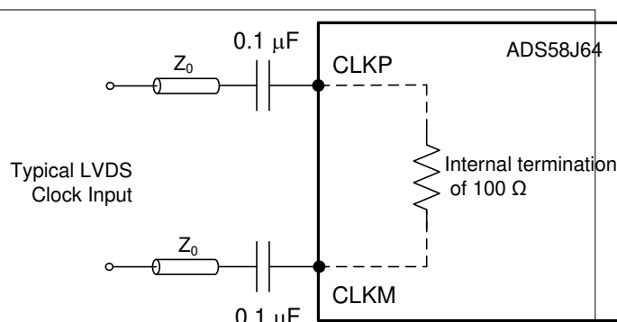
图 7-3. LVDS Clock Driving Circuit
