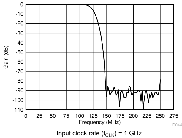
图 7-7. Decimation Filter Response vs Frequency
