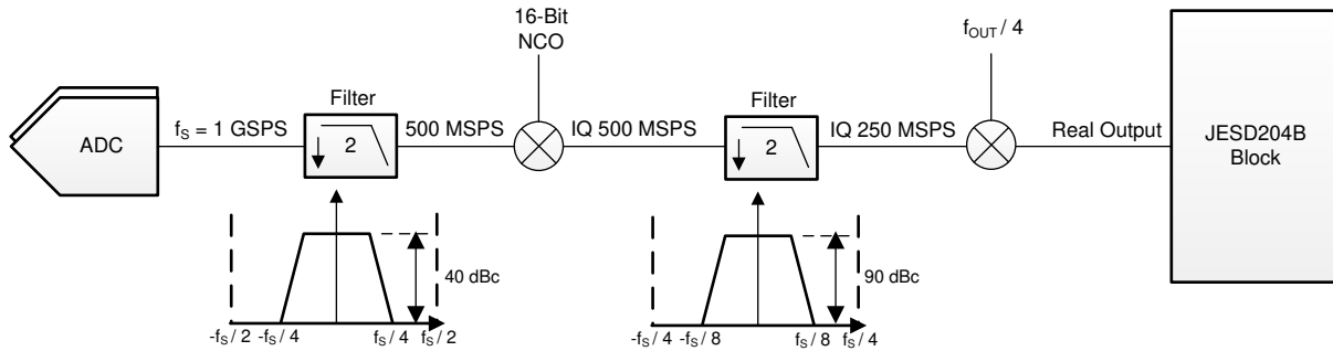
图 7-13. Operating Mode 4
