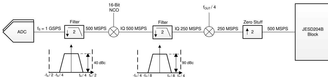
图 7-15. Operating Mode 7
