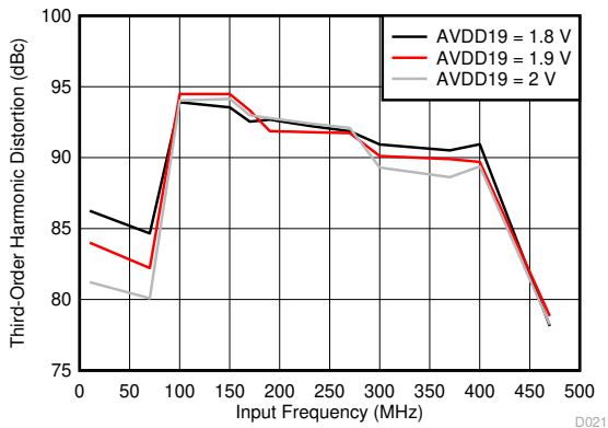
图 6-22. HD3 vs Input Frequency and AVDD19 Supply
