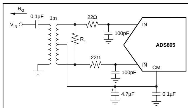
FIGURE 3. Transformer-Coupled Input.
