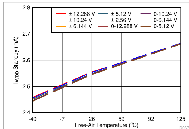
图 6-45. AVDD Current vs Temperature (Standby Mode)
