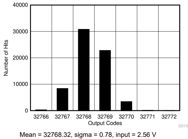
图 6-21. DC Histogram for Mid-Scale Inputs (0 V – 5.12 V)
