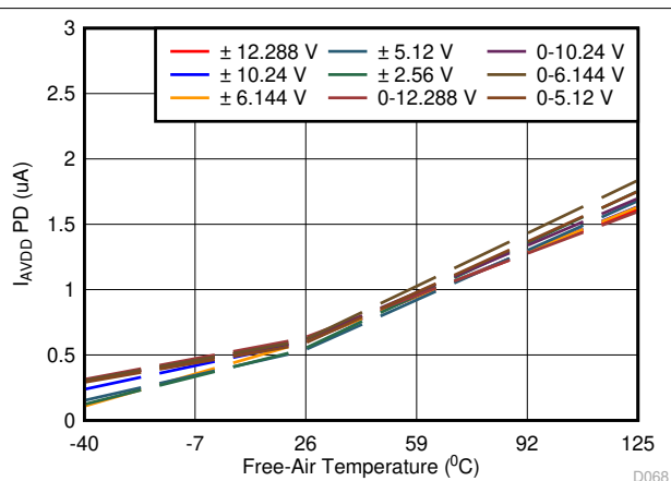
图 6-46. AVDD Current vs Temperature (Power-Down Mode)
