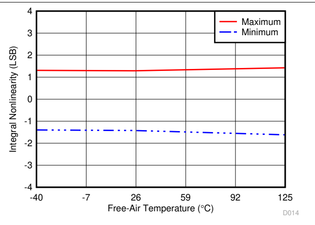
图 6-26. INL vs Temperature (All Bipolar Ranges)
