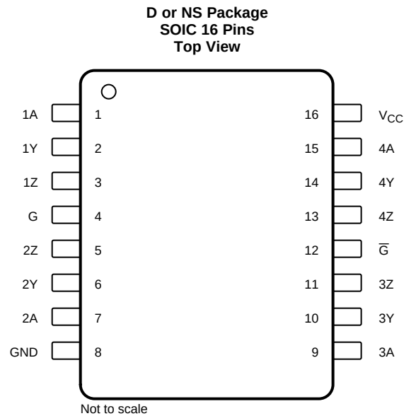
Pin Functions
