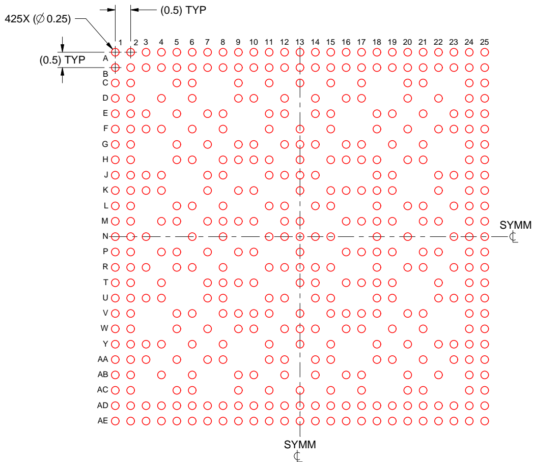
SOLDER PASTE EXAMPLE BASED ON 0.125 mm THICK STENCIL SCALE: 8X
