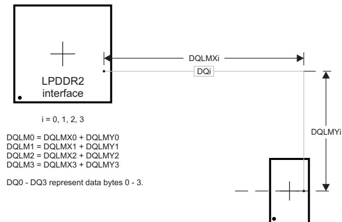
Figure 5-86. DQ[x] Routing
