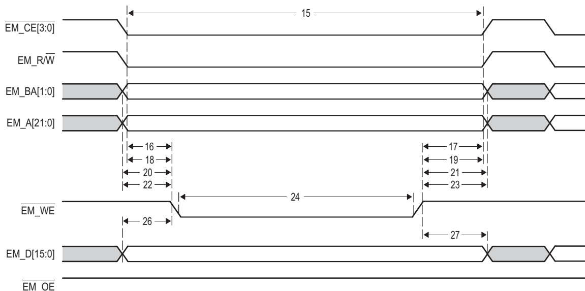
图 10-52. EMIF16 Asynchronous Memory Write Timing Diagram
