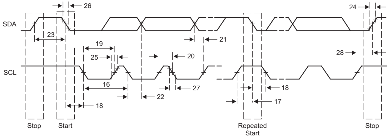
图 10-32. I²C Transmit Timings
