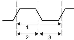
图 10-35. HyperLink Station Management Clock Timing
