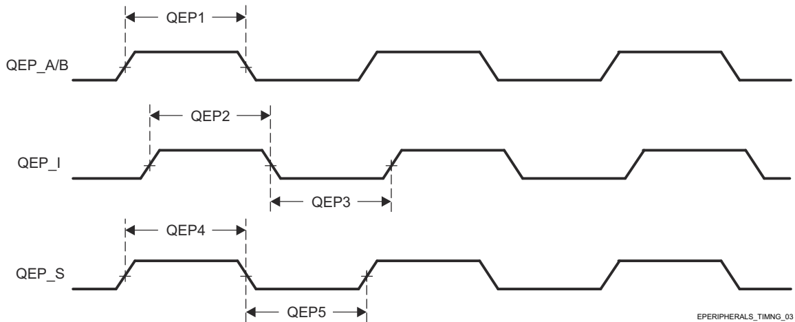
图 7-33. EQEP Timing Requirements
