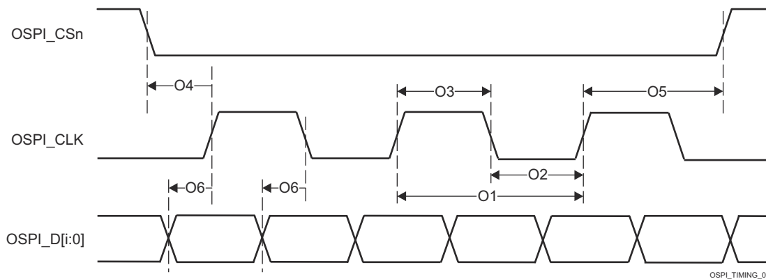
图 7-83. OSPI Switching Characteristics - DDR
