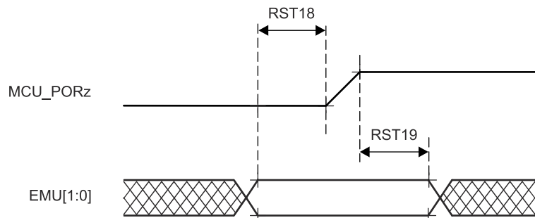
图 7-9. EMUx Timing Requirements
