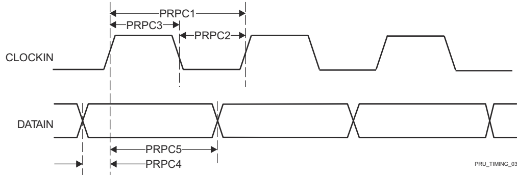
图 7-85. PRU_ICSSG PRU Parallel Capture Timing Requirements - Rising Edge Mode
