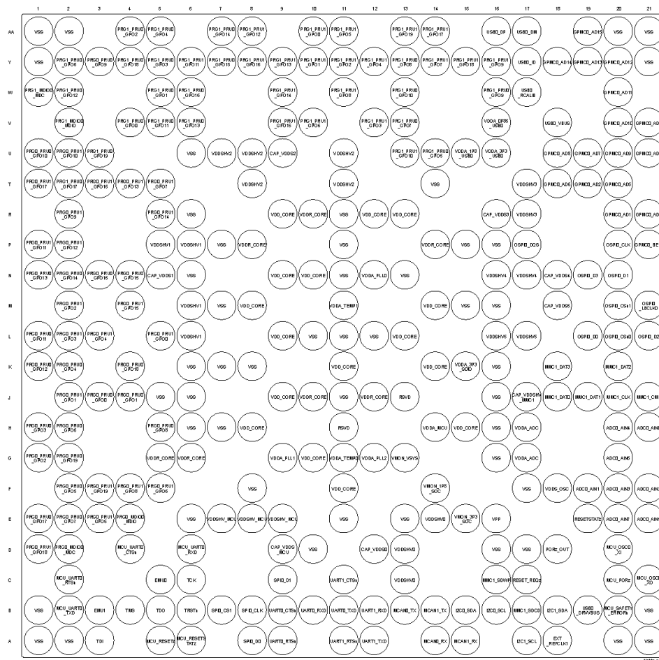
图 6-2. ALX FCBGA-N293 Pin Diagram (Bottom View)
