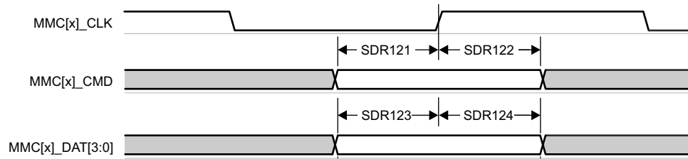
图 7-68. MMC1 - UHS-I SDR12 - Receive Mode
