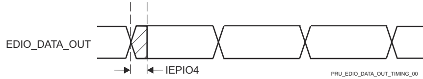
图 7-95. PRU_ICSSG IEP Digital IOs Timing Requirements
