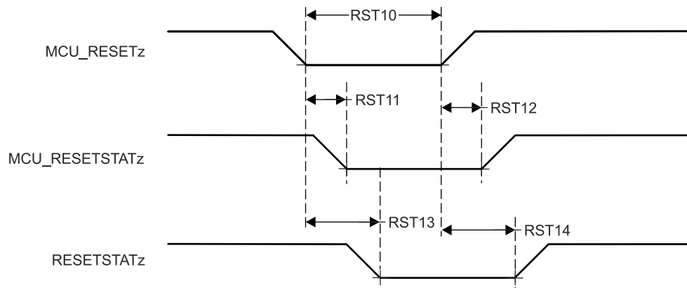
图 7-7. MCU_RESETz, MCU_RESETSTATz, and RESETSTATz Timing Requirements and Switching Characteristics
