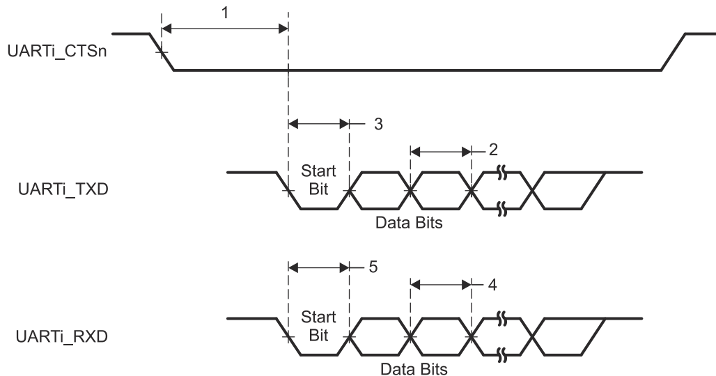
图 7-108. UART Timing Requirements and Switching Characteristics
