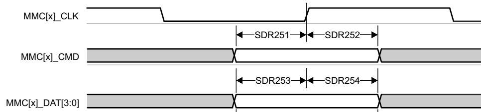
图 7-70. MMC1 - UHS-I SDR25 - Receive Mode
