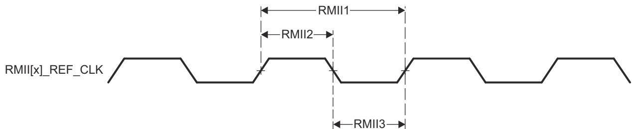
图 7-21. CPSW3G RMII[x]_REF_CLK Timing Requirements - RMII Mode
