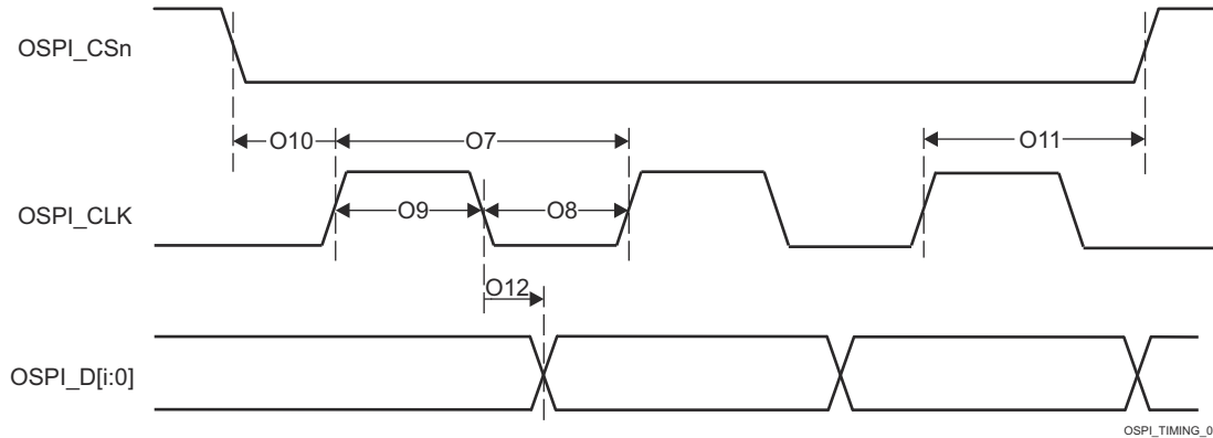
图 7-80. OSPI Switching Characteristics - SDR
