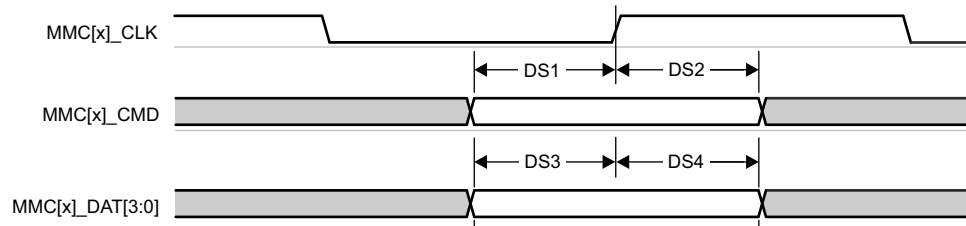
图 7-64. MMC1 - Default Speed - Receive Mode
