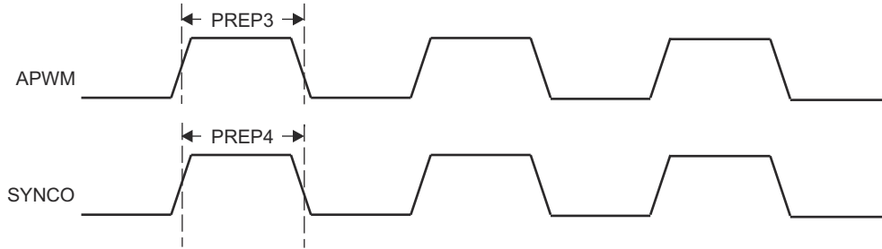
图 7-99. PRU_ICSSG ECAP Switching Characteristics
