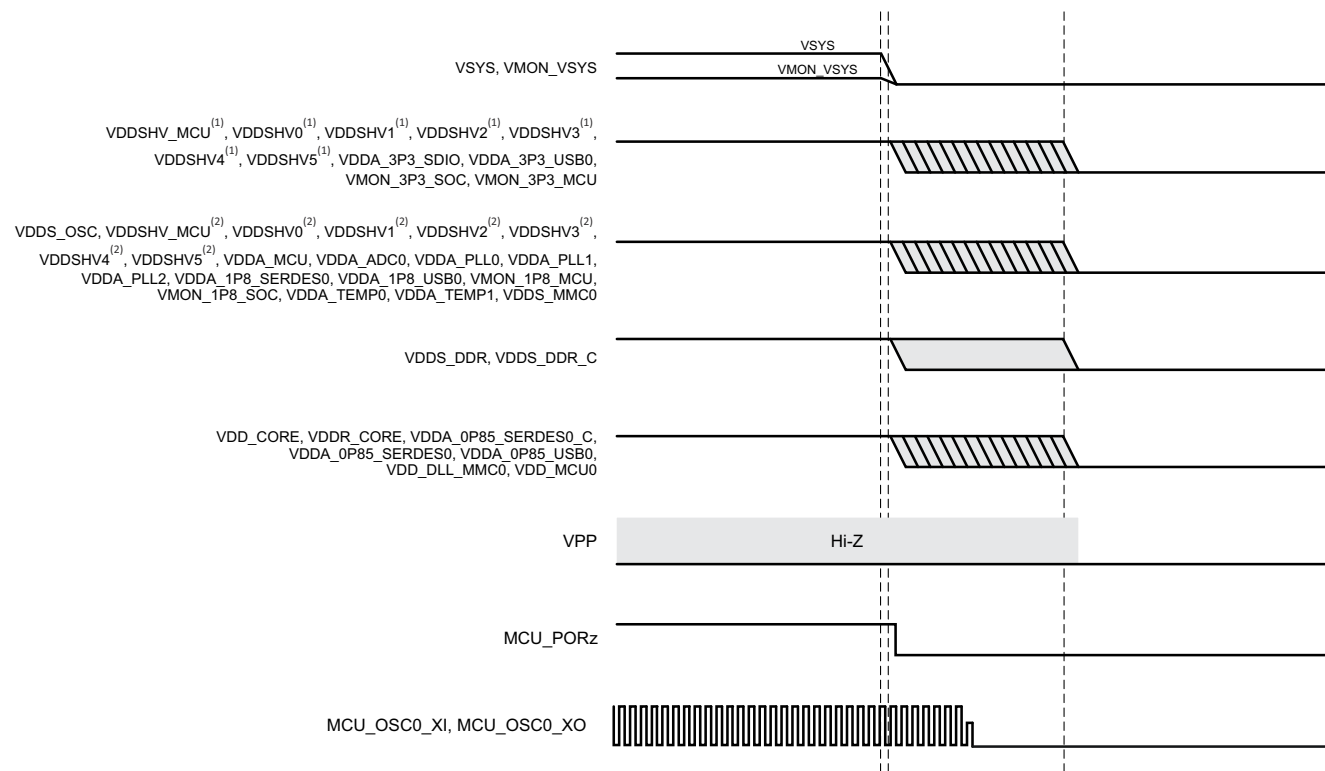
图 7-4. Power-Down Sequencing
