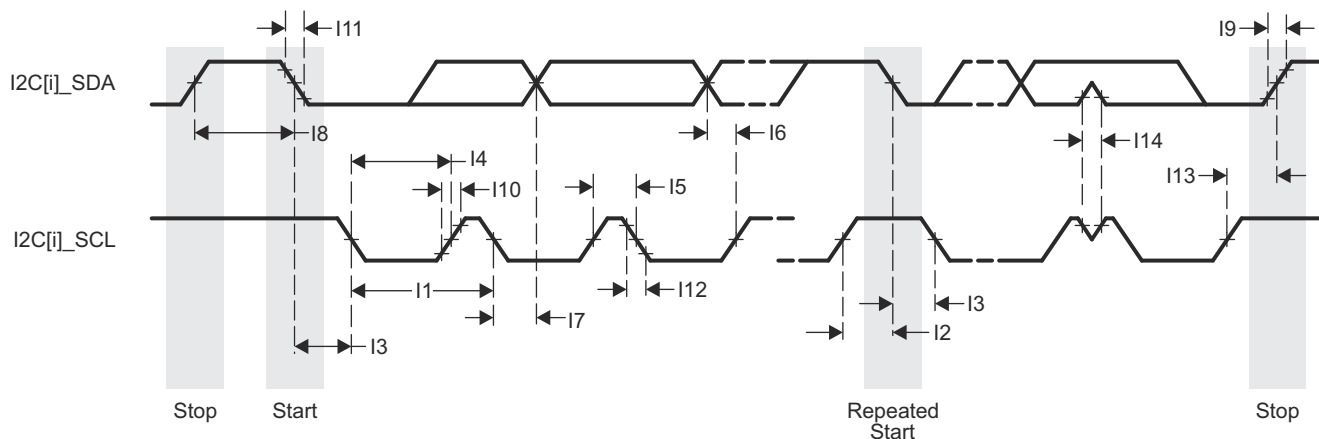
图 7-52. I2C Receive Timing
