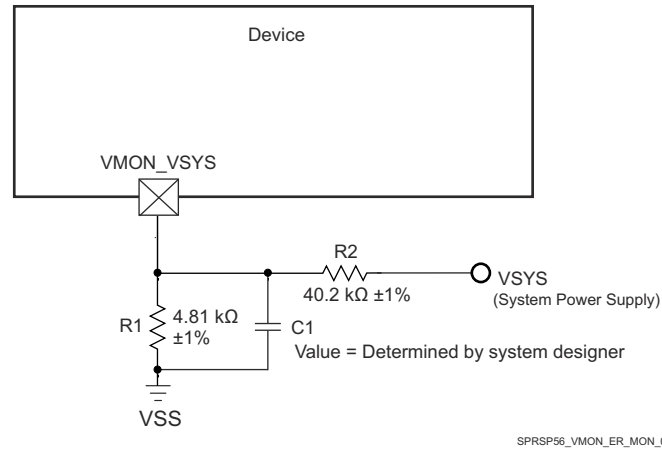
图 9-6. System Supply Monitor Voltage Divider Circuit
