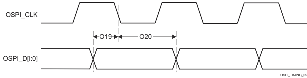
图 7-78. OSPI Timing Requirements - SDR, No Loopback Clock and Internal Pad Loopback Clock
