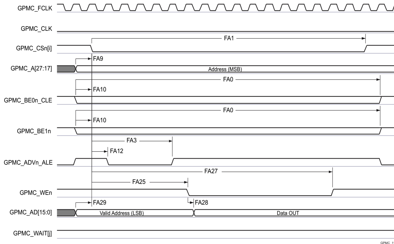
图 7-47. GPMC and Multiplexed NOR Flash — Asynchronous Write — Single Word
