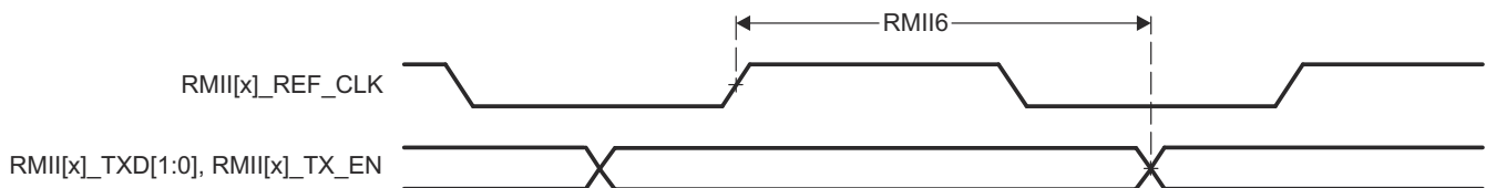
图 7-23. RMII[x]_TXD[1:0], and RMII[x]_TX_EN Switching Characteristics - RMII Mode
