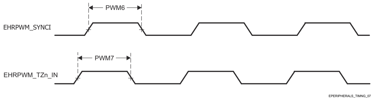
图 7-29. EPWM Timing Requirements
