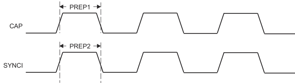
图 7-98. PRU_ICSSG ECAP Timing
