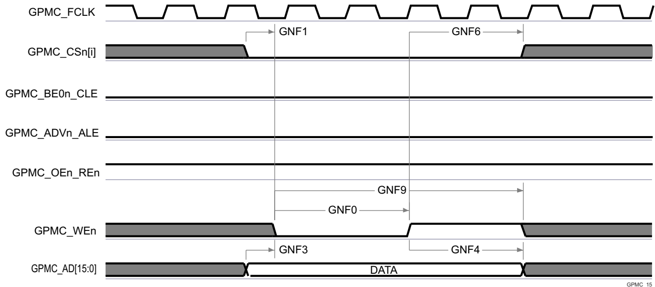
图 7-50. GPMC and NAND Flash — Data Read Cycle
