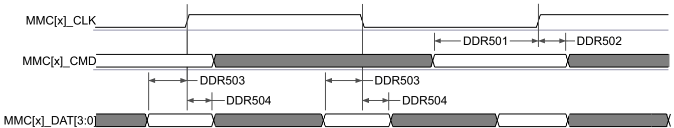
图 7-73. MMC1 - UHS-I DDR50 - Receive Mode
