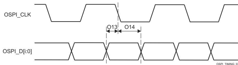
图 7-81. OSPI Timing Requirements - DDR, No Loopback Clock and Internal Pad Loopback Clock
