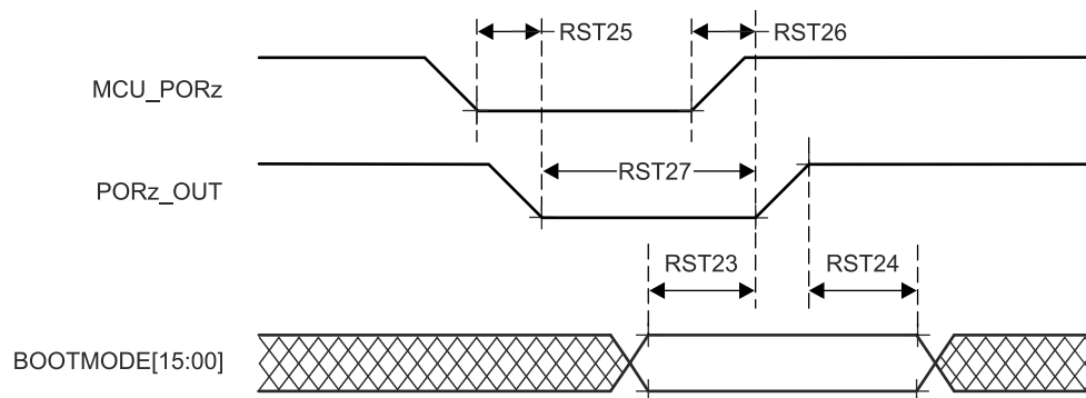
图 7-10. BOOTMODE Timing Requirements and PORz_OUT Switching Characteristics
