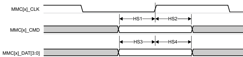
图 7-66. MMC1 - High Speed - Receive Mode
