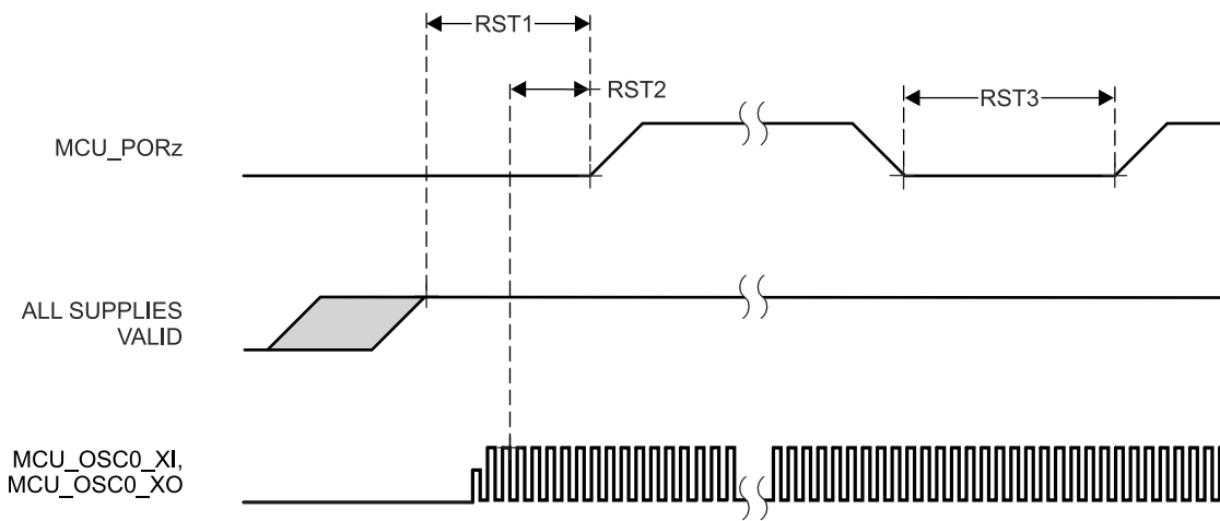
图 7-5. MCU_PORz Timing Requirements
