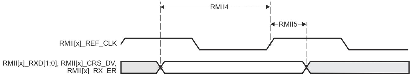
图 7-22. CPSW3G RMII[x]_RXD[1:0], RMII[x]_CRS_DV, RMII[x]_RX_ER Timing Requirements - RMII Mode
