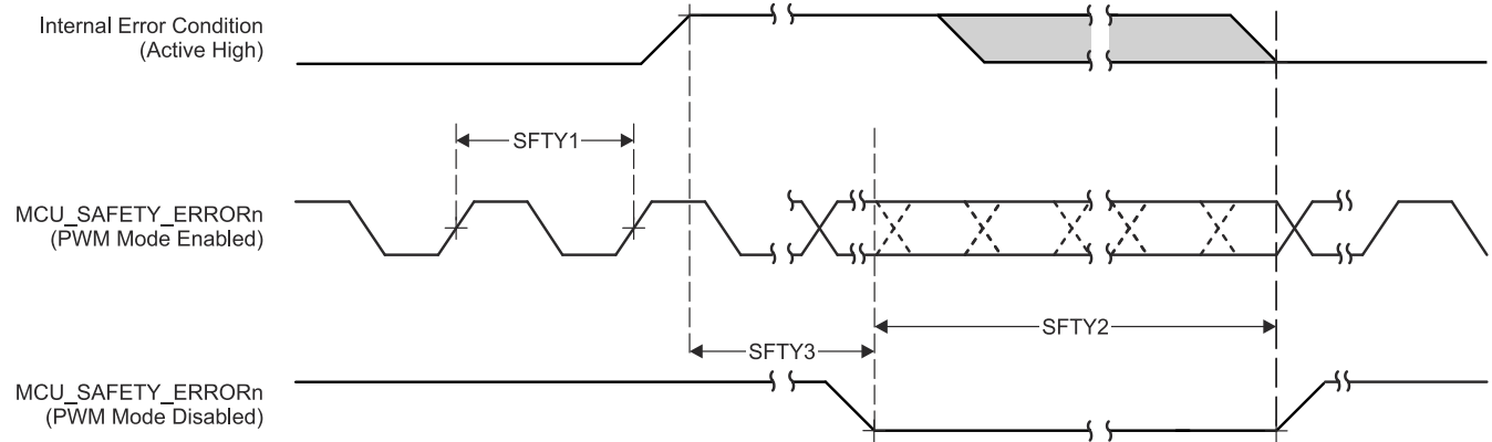
图 7-11. MCU_SAFETY_ERRORn Timing Requirements and Switching Characteristics
