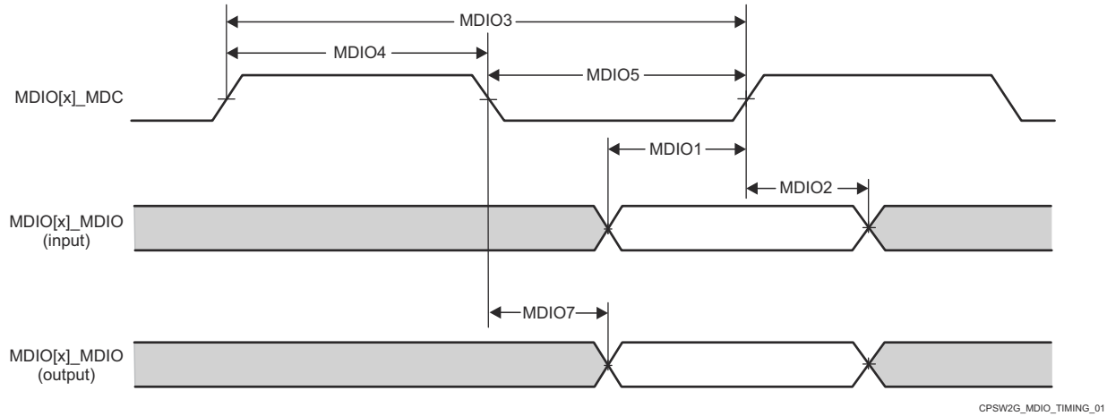
图 7-100. PRU_ICSSG MDIO Timing Requirements and Switching Characteristics
