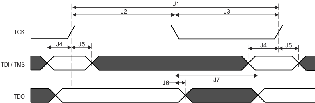
图 7-110. JTAG Timing Requirements and Switching Characteristics
