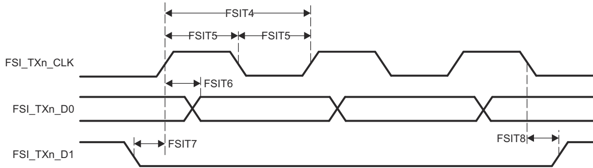
图 7-36. FSI Switching Characteristics - SPI Mode
