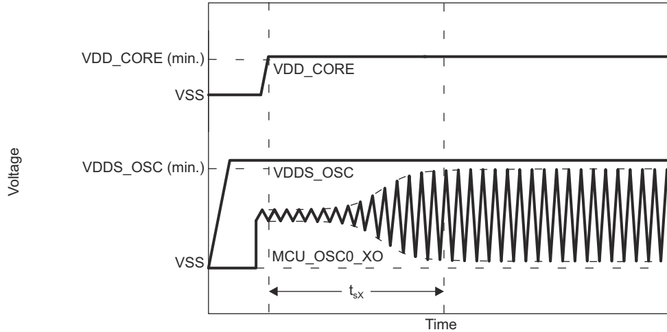
图 7-16. MCU_OSC0 Start-up Time
