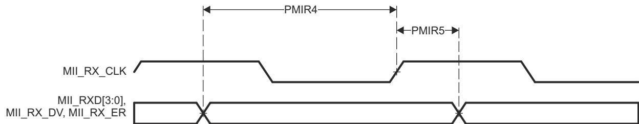
图 7-102. PRU_ICSSG MII[x]_RXD[3:0], MII[x]_RX_DV, and MII[x]_RX_ER Timing
