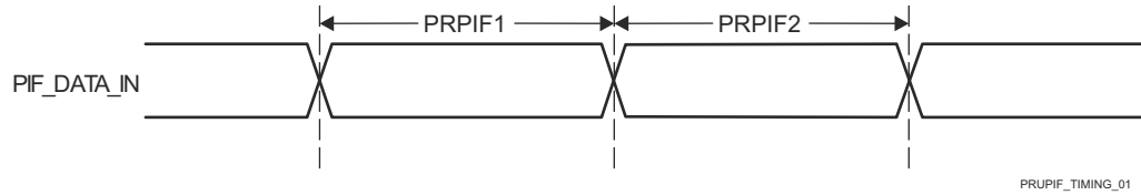
图 7-91. PRU_ICSSG PRU Peripheral Interface Timing Requirements
