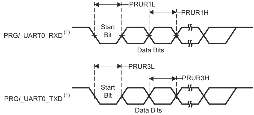
图 7-97. PRU_ICSSG UART Timing Requirements and Switching Characteristics
