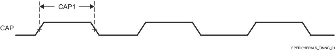
图 7-27. ECAP Timings Requirements
