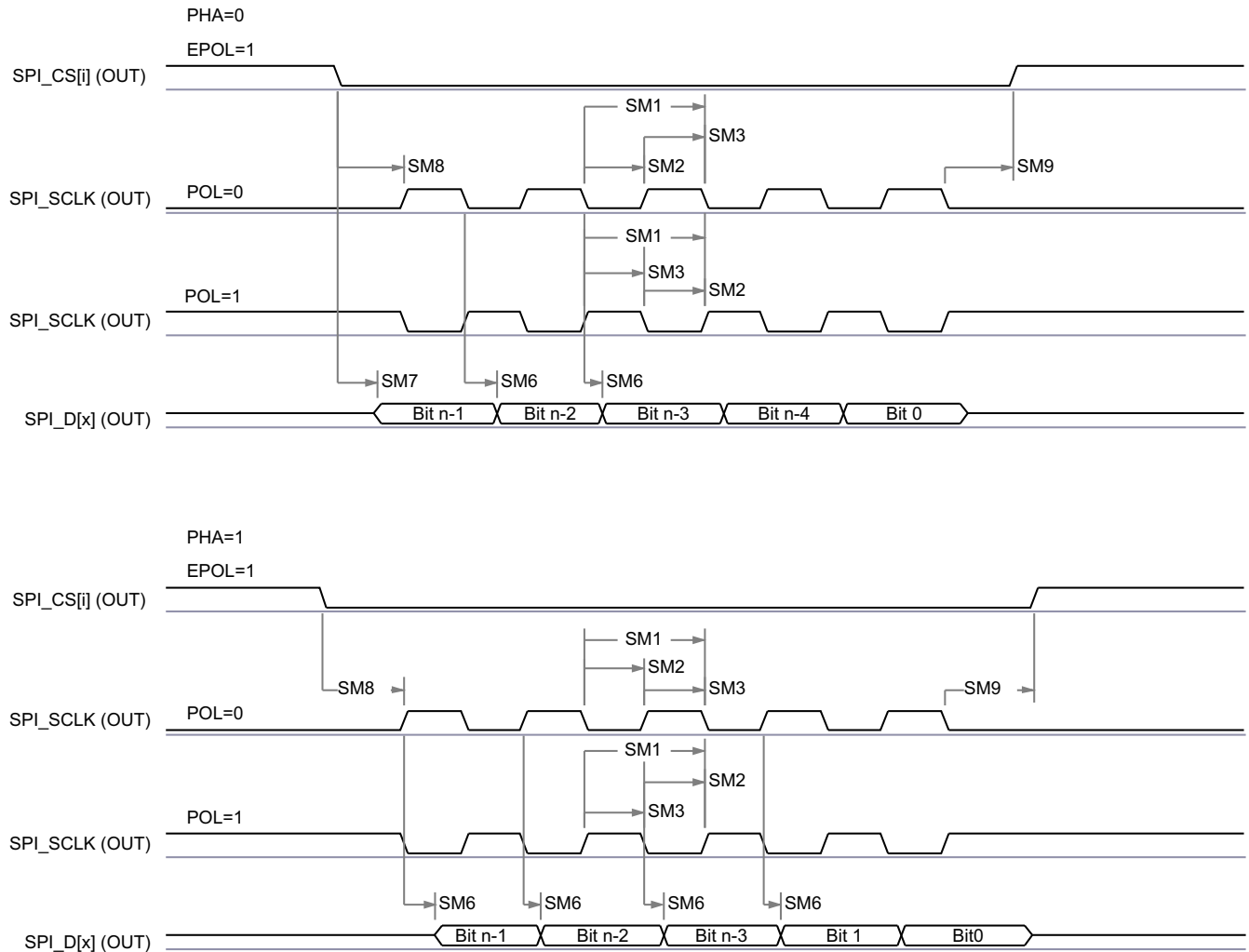
图 7-54. SPI Master Mode Transmit Timing
