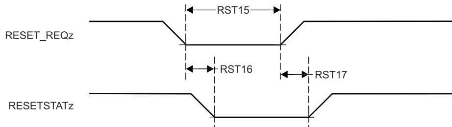
图 7-8. RESET_REQz and RESETSTATz Timing Requirements and Switching Characteristics
