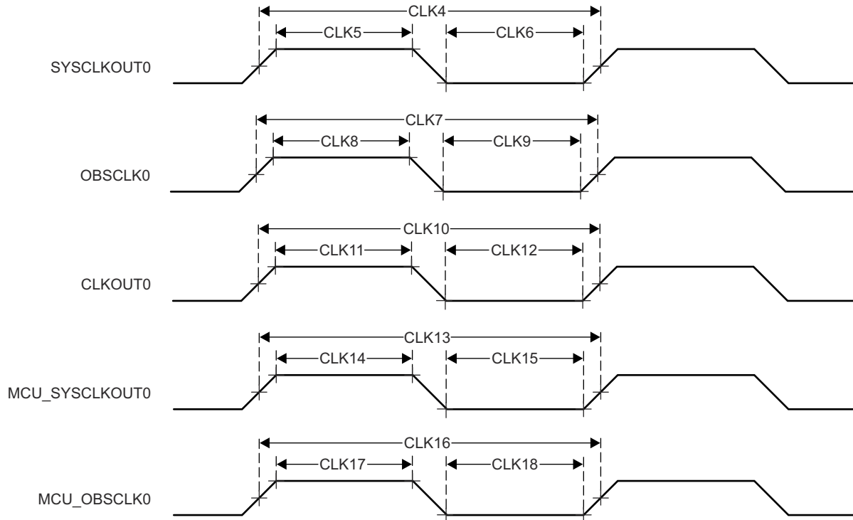
图 7-13. Clock Switching Characteristics
