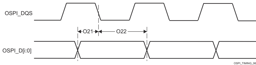
图 7-79. OSPI Timing Requirements - SDR, External Loopback Clock
