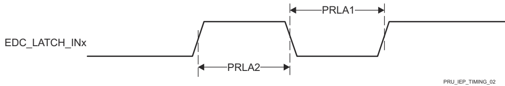
图 7-96. PRU_ICSSG IEP LATCH_INx Timing Requirements
