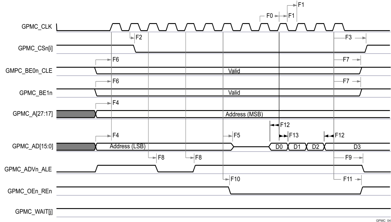
图 7-39. GPMC and NOR Flash—Synchronous Burst Write (GPMCFCLKDIVIDER = 0)
