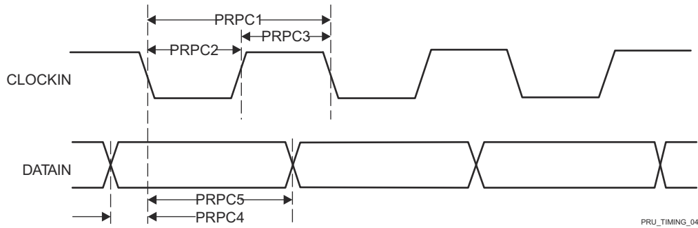
图 7-86. PRU_ICSSG PRU Parallel Capture Timing Requirements - Falling Edge Mode
