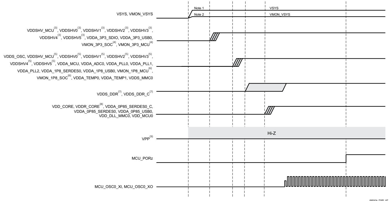
图 7-3. Power-Up Sequencing
