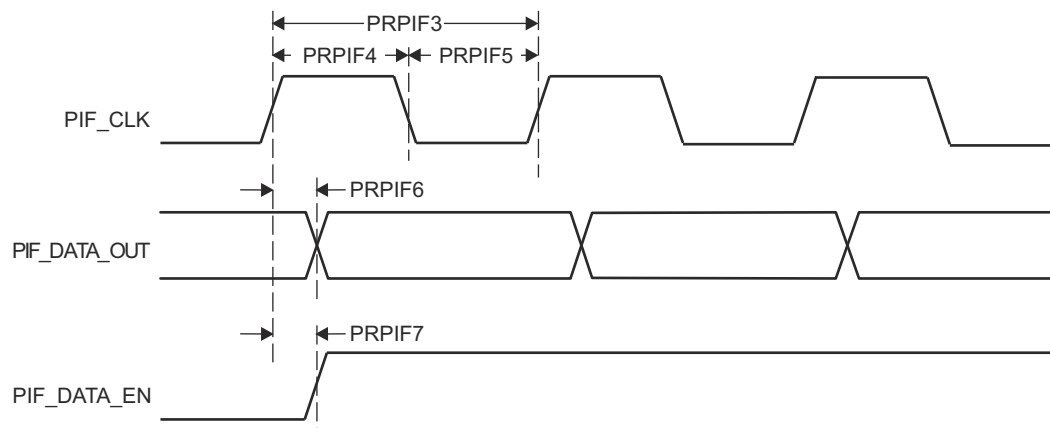
图 7-92. PRU_ICSSG PRU Peripheral Interface Switching Characteristics
