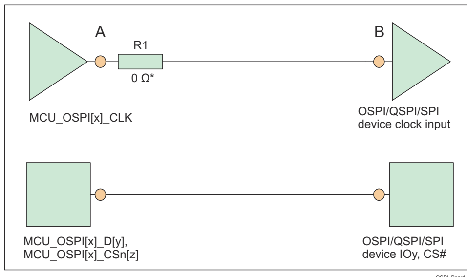
图 9-2. OSPI Interface High Level Schematic
