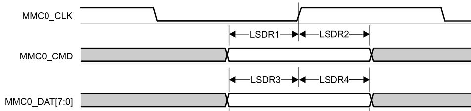
图 7-57. MMC0 – Legacy SDR – Receive Mode
