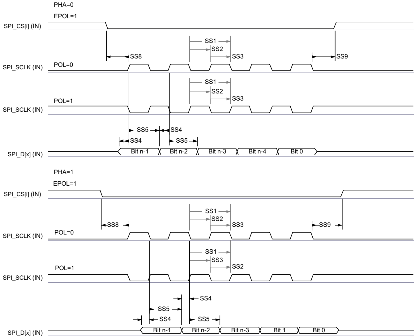
图 7-55. SPI Slave Mode Receive Timing
