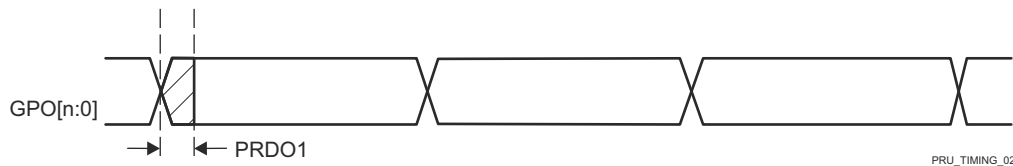
图 7-84. PRU_ICSSG PRU Direct Output Timing
