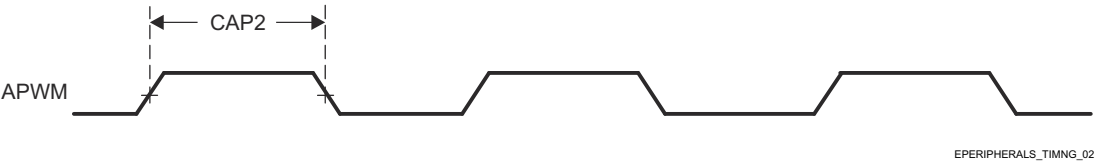
图 7-28. ECAP Switching Characteristics
