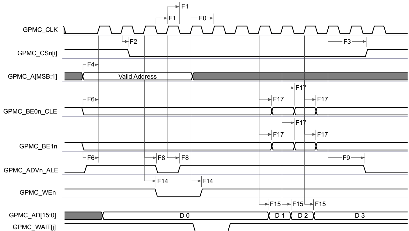
图 7-38. GPMC and NOR Flash — Synchronous Burst Read — 4x16 - bit (GPMCFCLKDIVIDER = 0)
