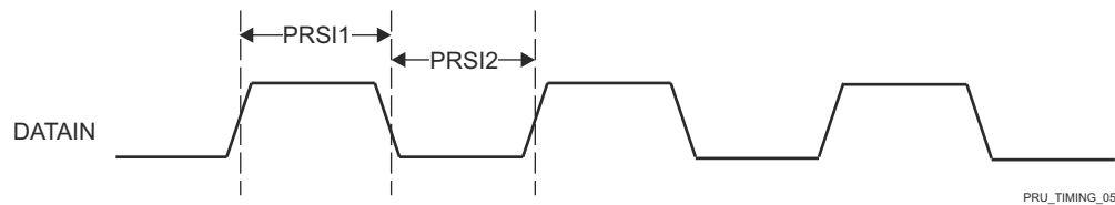
图 7-87. PRU_ICSSG PRU Shift In Timing
