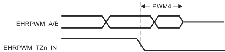
图 7-32. EHRPWM_TZn_IN to EHRPWM_A/B Hi-Z Switching Characteristics
