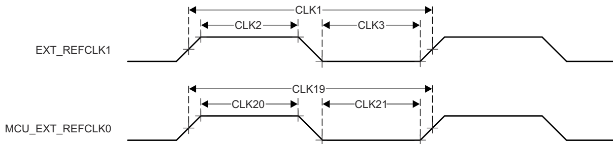
图 7-12. Clock Timing Requirements
