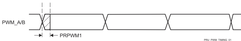
图 7-93. PRU_ICSSG PWM Timing
