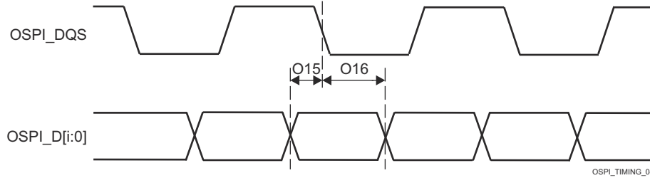
图 7-82. OSPI Timing Requirements - DDR, External Loopback Clock and DQS
