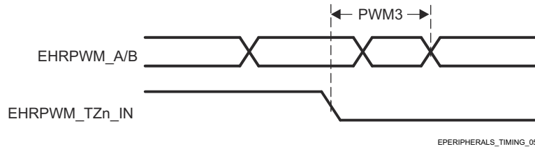
图 7-31. EHRPWM_TZn_IN to EHRPWM_A/B Forced Switching Characteristics
