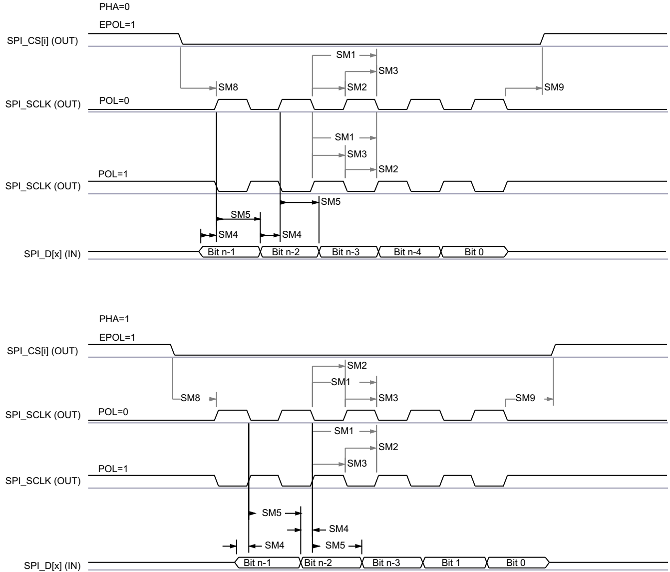
图 7-53. SPI Master Mode Receive Timing
