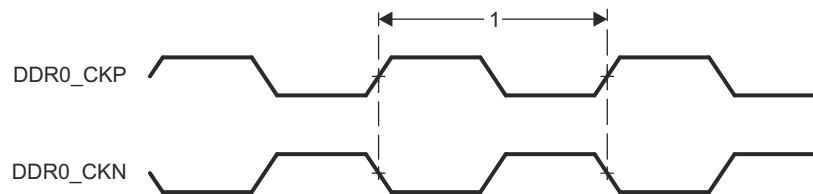
图 7-26. DDRSS Switching Characteristics
