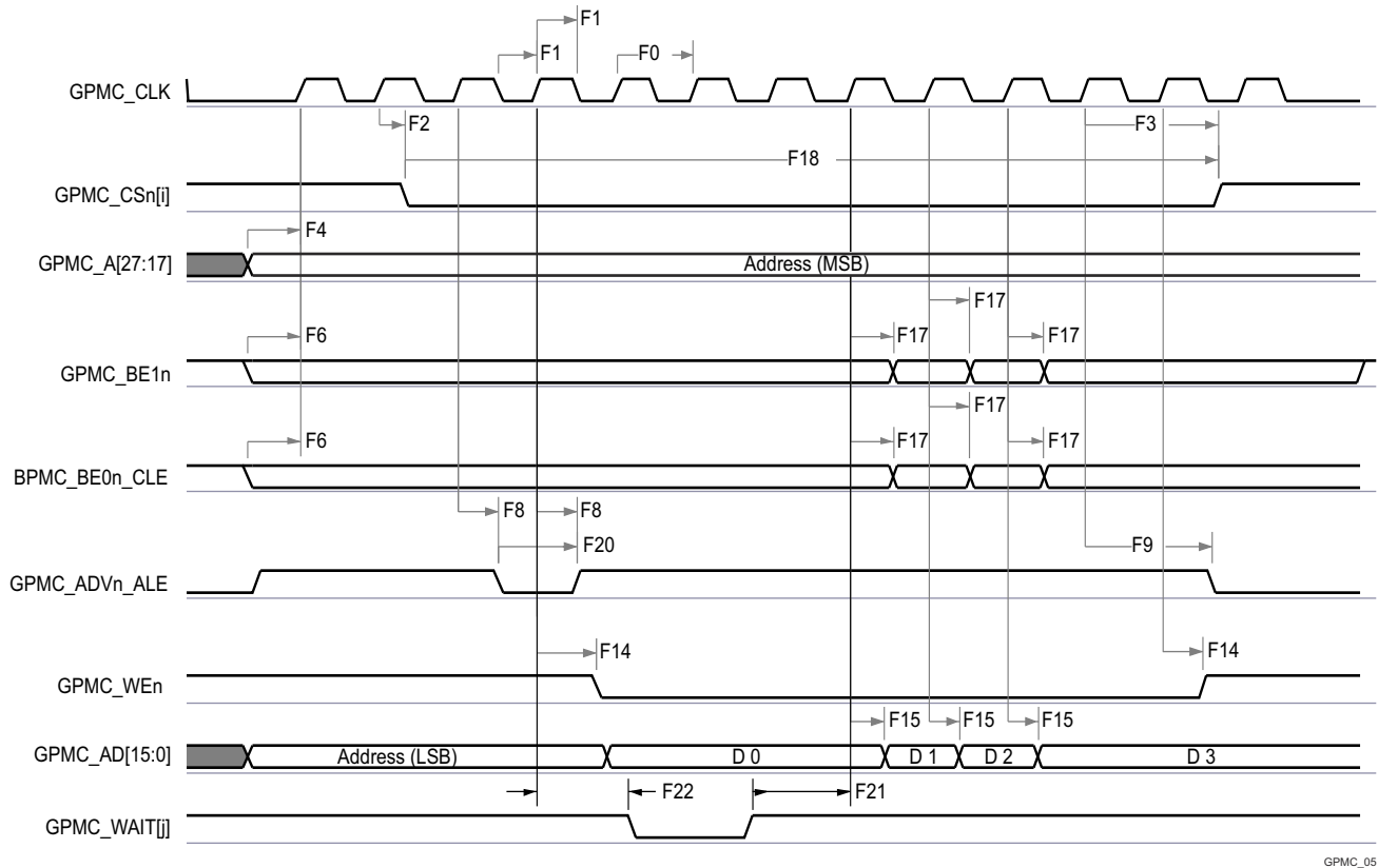
图 7-41. GPMC and Multiplexed NOR Flash — Synchronous Burst Write
