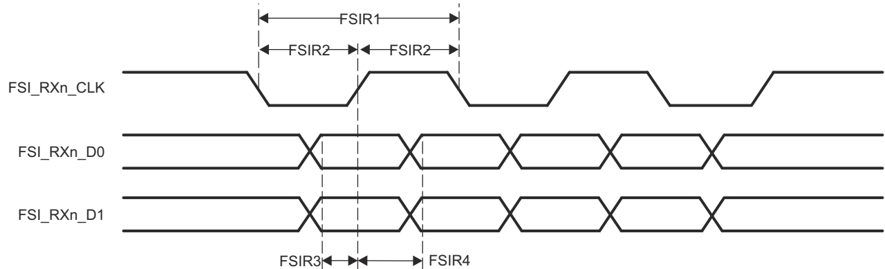
图 7-34. FSI Timing Requirements
