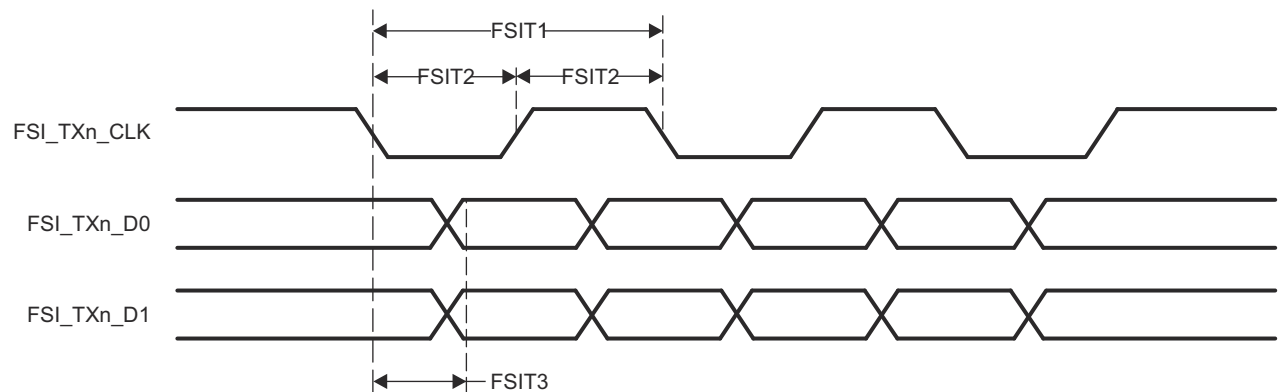
图 7-35. FSI Switching Characteristics - FSI Mode
