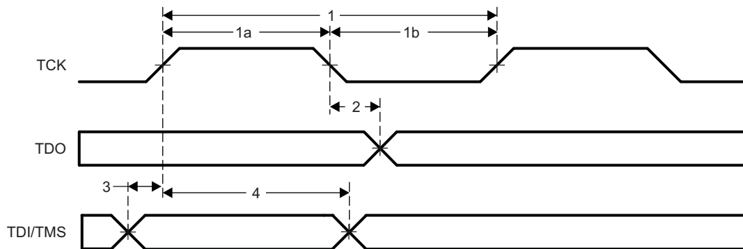
Figure 5-146. JTAG Timing
