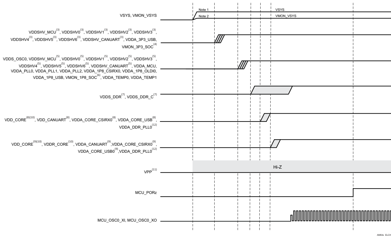
Figure 7-5. Power-Up Sequencing
