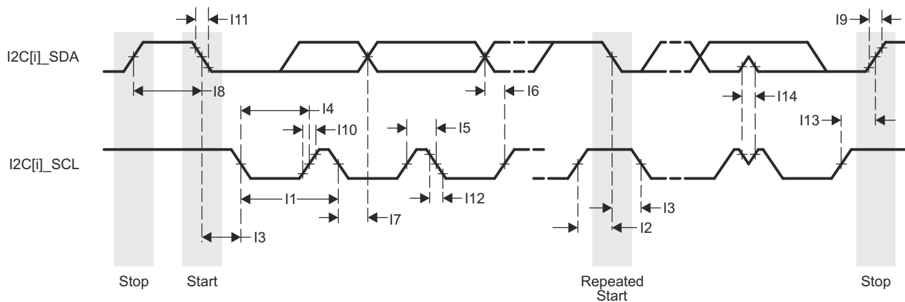
图 7-52. I2C Receive Timing
