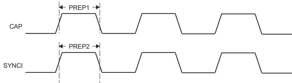
图 7-98. PRU_ICSSG ECAP Timing
