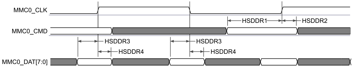
图 7-61. MMC0 - High Speed DDR Mode - Receive Mode
