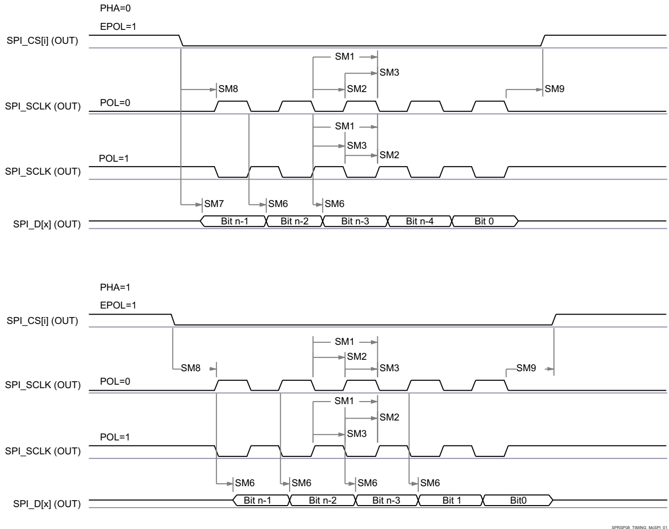
图 7-54. SPI Master Mode Transmit Timing
