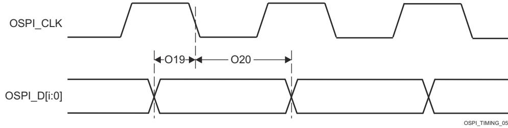
图 7-78. OSPI Timing Requirements - SDR, No Loopback Clock and Internal Pad Loopback Clock
