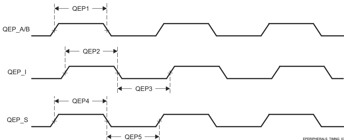
Figure 7-44. EQEP Timing Requirements
