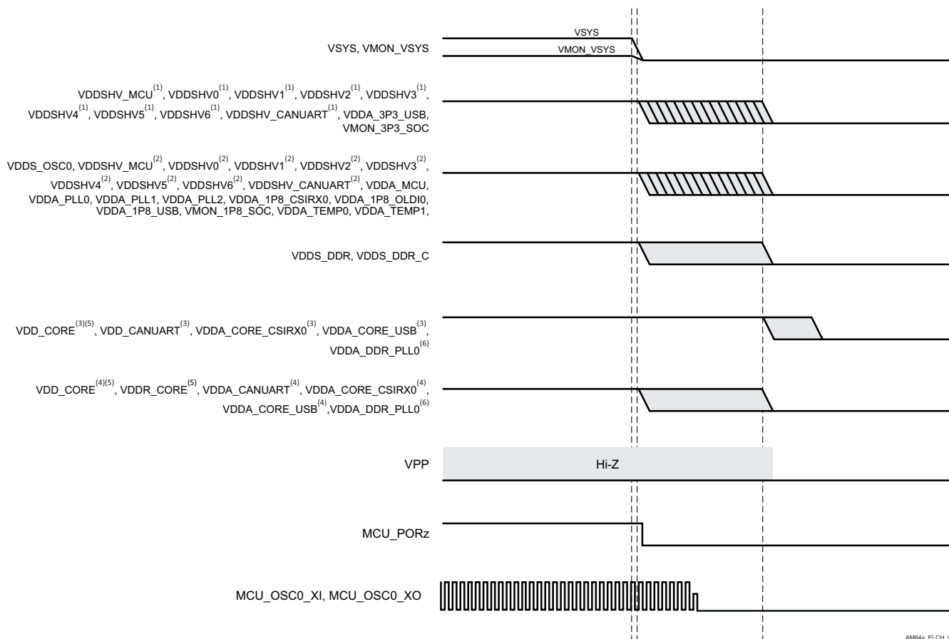
Figure 7-6. Power-Down Sequencing
