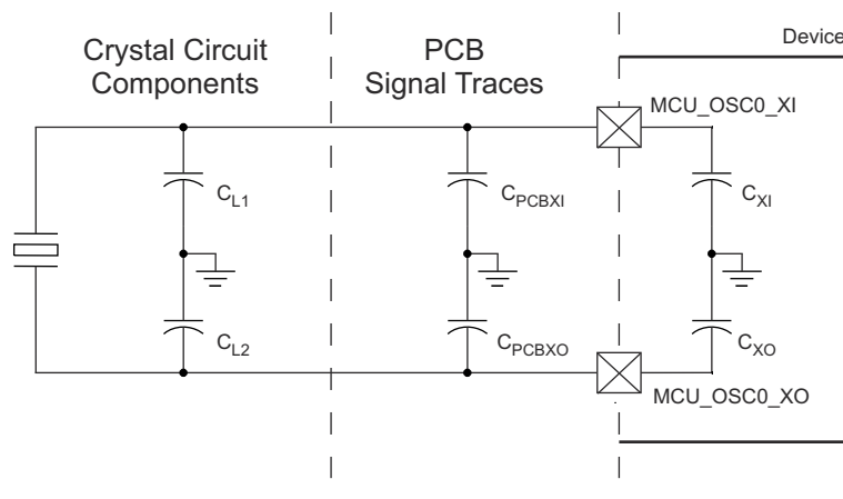
Figure 7-18. Load Capacitance
