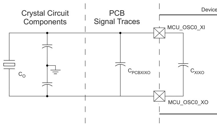
Figure 7-19. Shunt Capacitance
