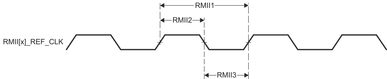
Figure 7-26. CPSW3G RMII[x]_REF_CLK Timing Requirements – RMII Mode
