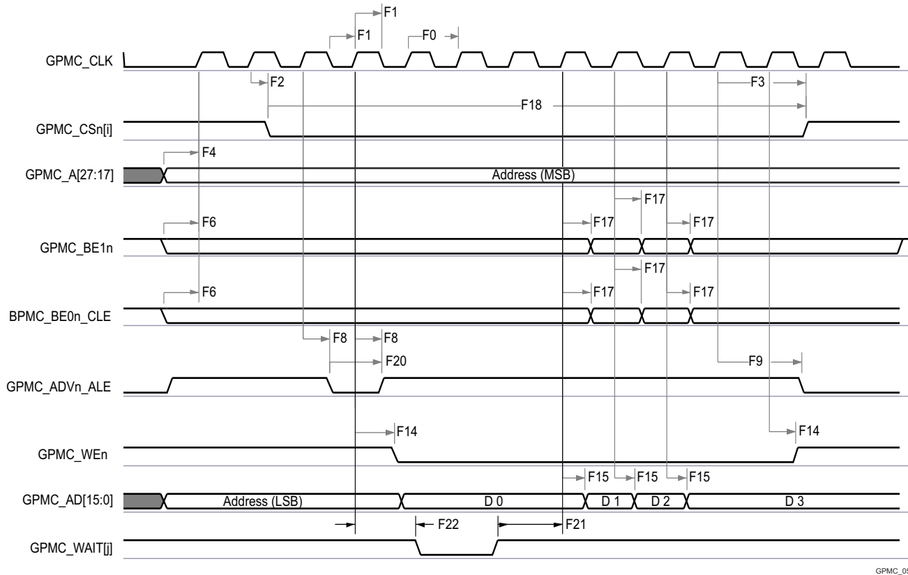
Figure 7-49. GPMC and Multiplexed NOR Flash — Synchronous Burst Write
