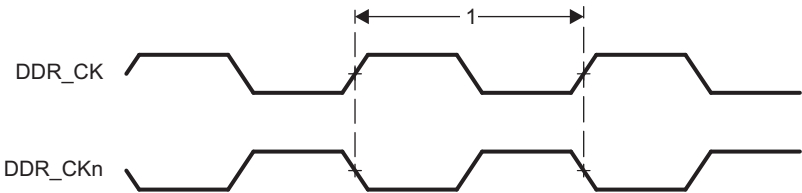
图 7-38. DDR2 Memory Interface Clock Timing
