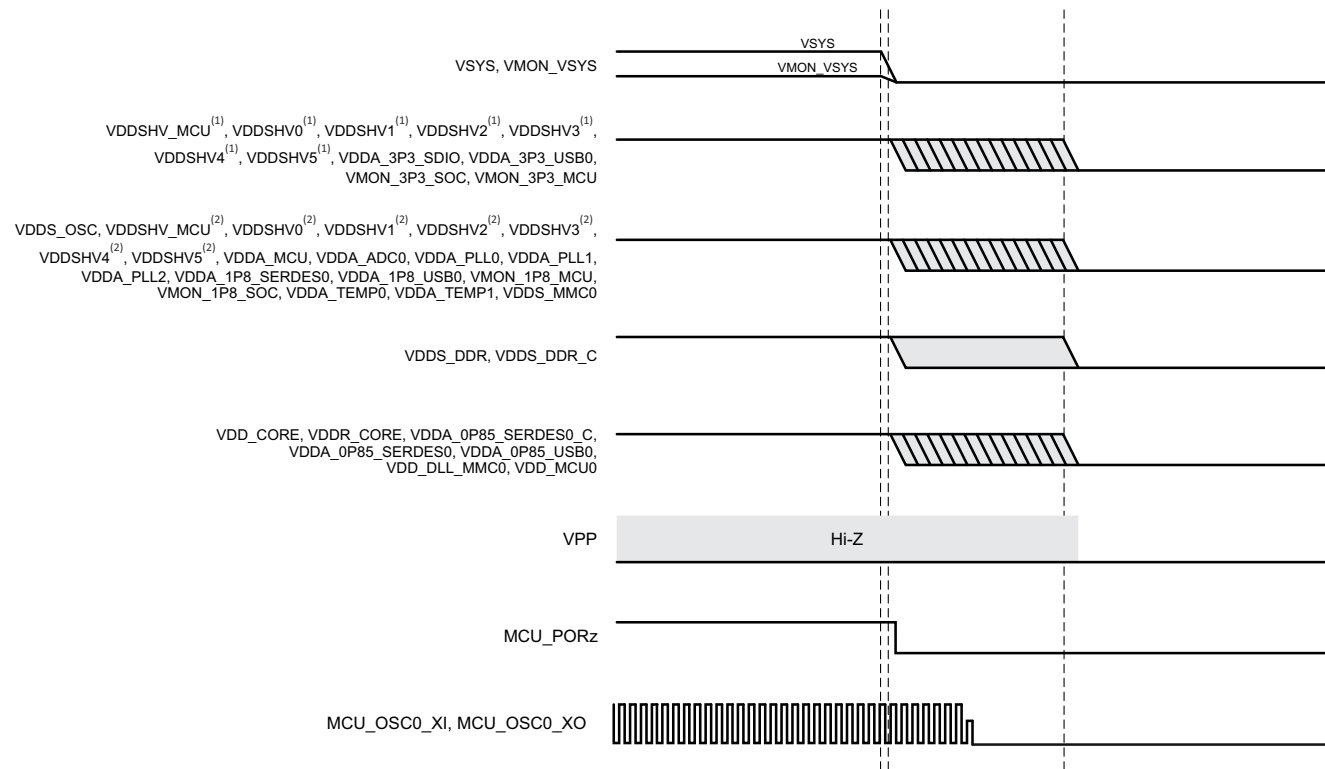
图 7-4. Power-Down Sequencing
