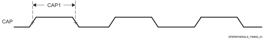
图 7-27. ECAP Timings Requirements
