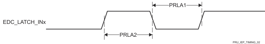
图 7-96. PRU_ICSSG IEP LATCH_INx Timing Requirements
