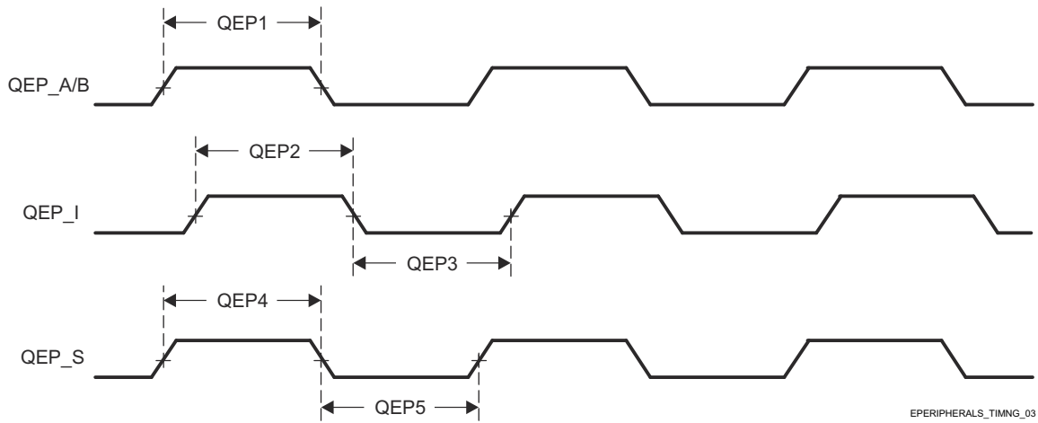
图 7-33. EQEP Timing Requirements
