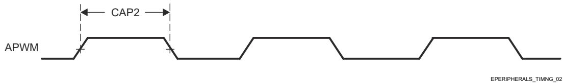
图 7-28. ECAP Switching Characteristics
