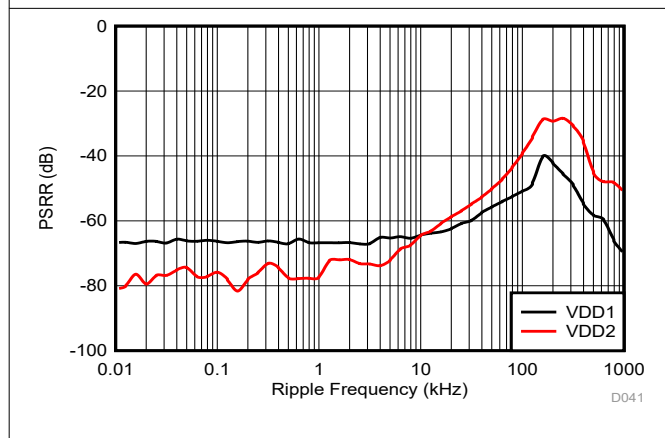
图 6-31. Power-Supply Rejection Ratio vs Ripple Frequency
