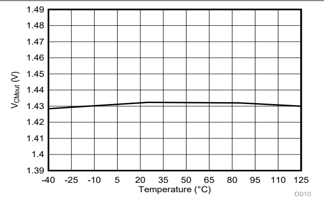
图 6-34. Common-Mode Output Voltage vs Temperature
