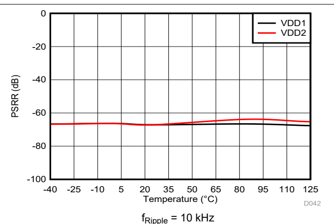
图 6-32. Power-Supply Rejection Ratio vs Temperature
