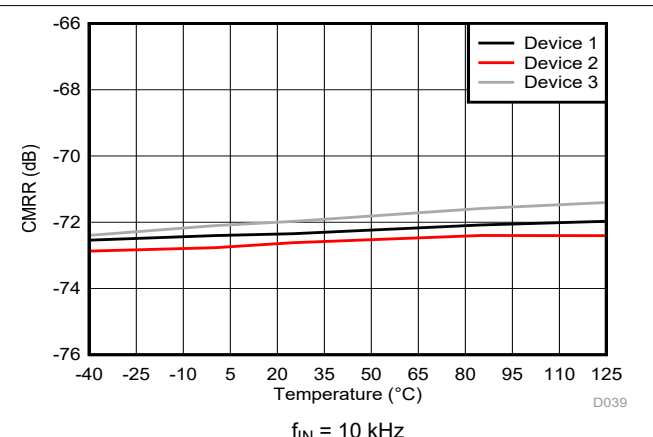
图 6-30. Common-Mode Rejection Ratio vs Temperature
