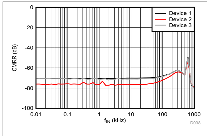
图 6-29. Common-Mode Rejection Ratio vs Input Frequency
