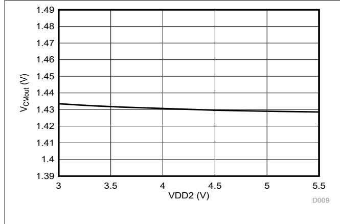
图 6-33. Common-Mode Output Voltage vs Supply Voltage
