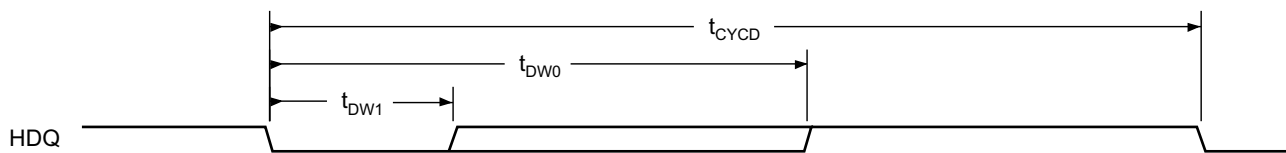
图 5-40. Device HDQ Interface Bit Write Timing (Command / Address or Data)
