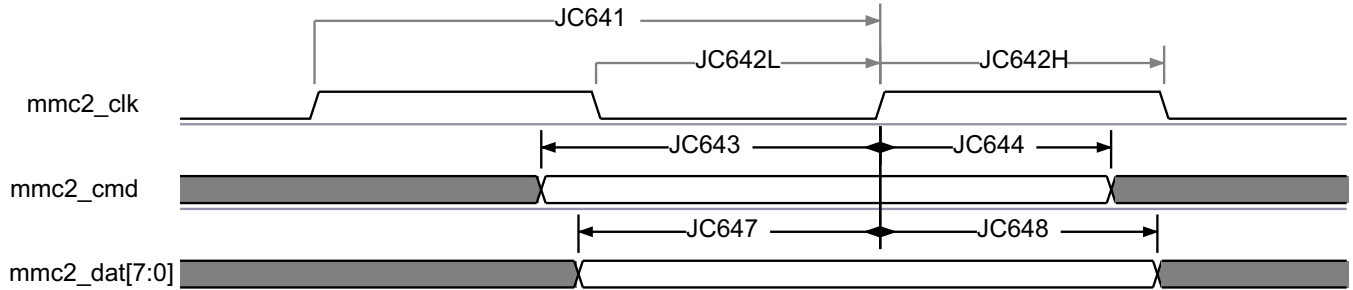
图 5-89. MMC/SD/SDIO in - High Speed JC64 - Receiver Mode
