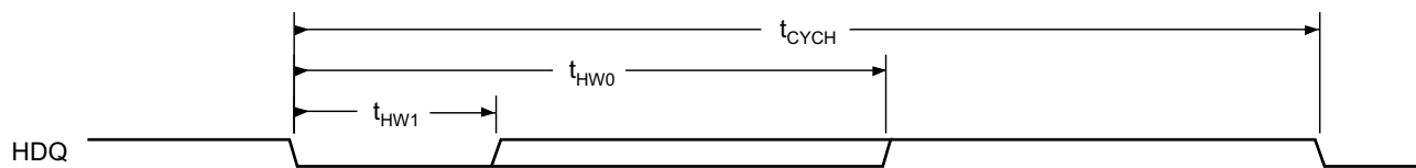
图 5-39. Device HDQ Interface Bit Read Timing (Data)
