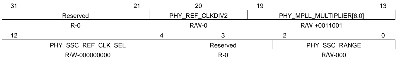
图 8-39. USB_PHY_CTL5 Register
