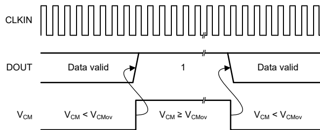
图 7-6. Output of the AMC1306M05-Q1 in Case of a Common-Mode Overage
