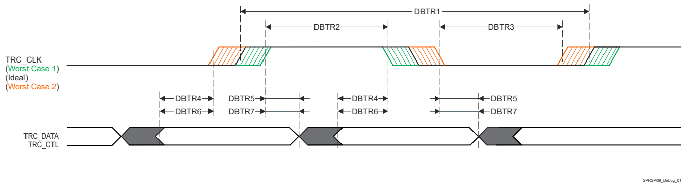
图 7-124. Debug Trace Switching Characteristics
