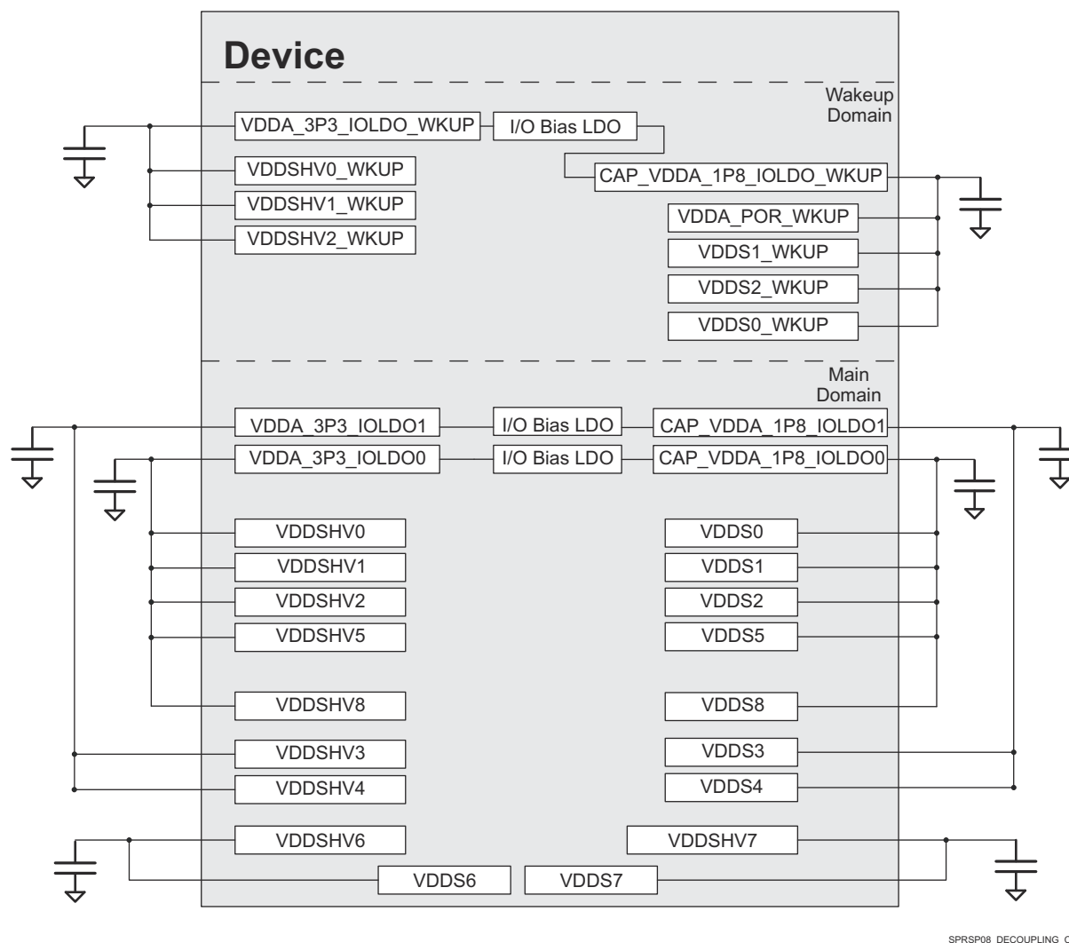
图 9-7. All VDDSHV[8:0], and VDDSHV[2:0]_WKUP Supplies Configured for 3.3 V Operation
