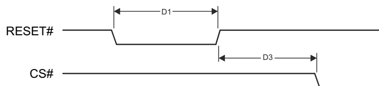
图 7-64. HyperBus Timing Diagrams - Receiver Mode
