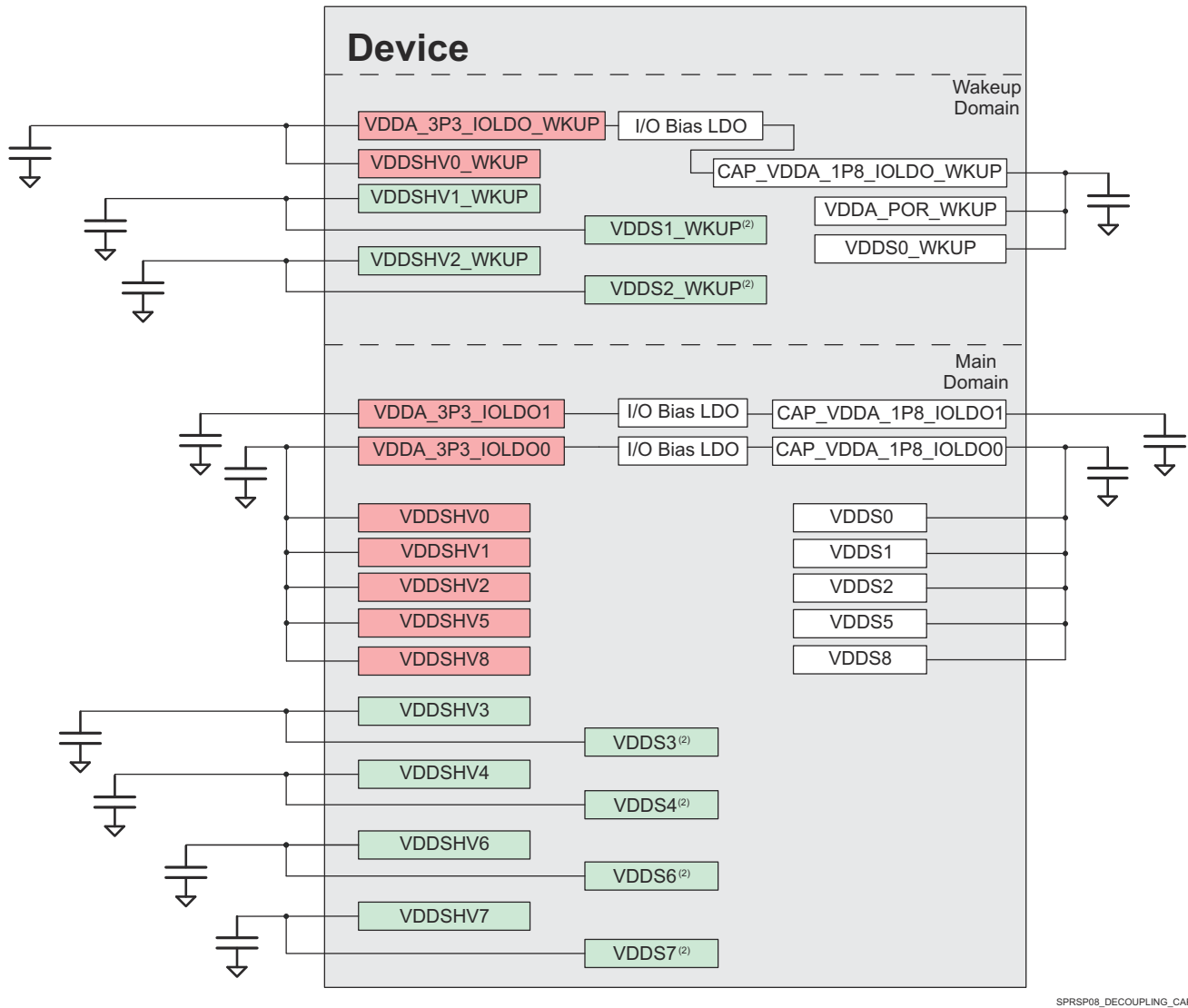
图 9-9. VDDSHV[8:0] and VDDSHV[2:0]_WKUP Supplies Configured for Combination of 1.8 V or 3.3 V Operation
