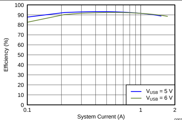
Charge Disabled SYS loaded V_{BATREG} = 3.6V USB1500 ILIM
