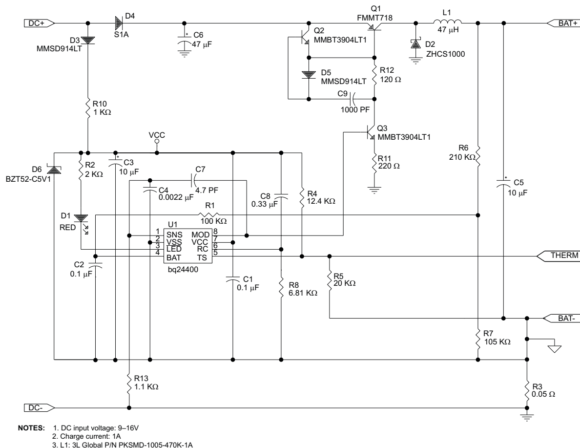
Figure 8. 3-Cell NiCd/NiMH 1A Charger
