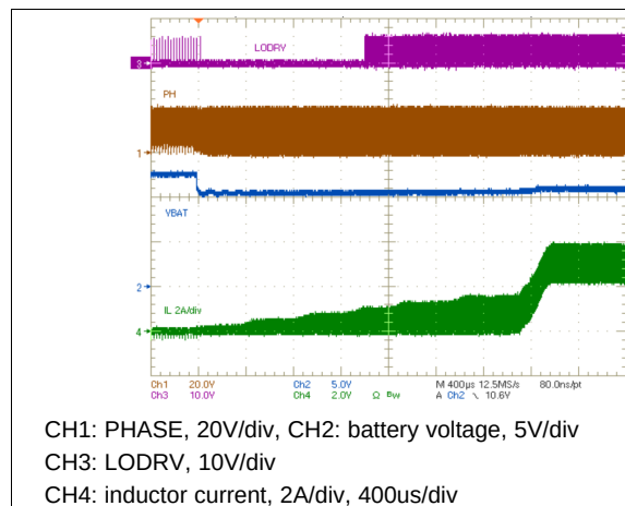
Figure 23. Battery Insertion
