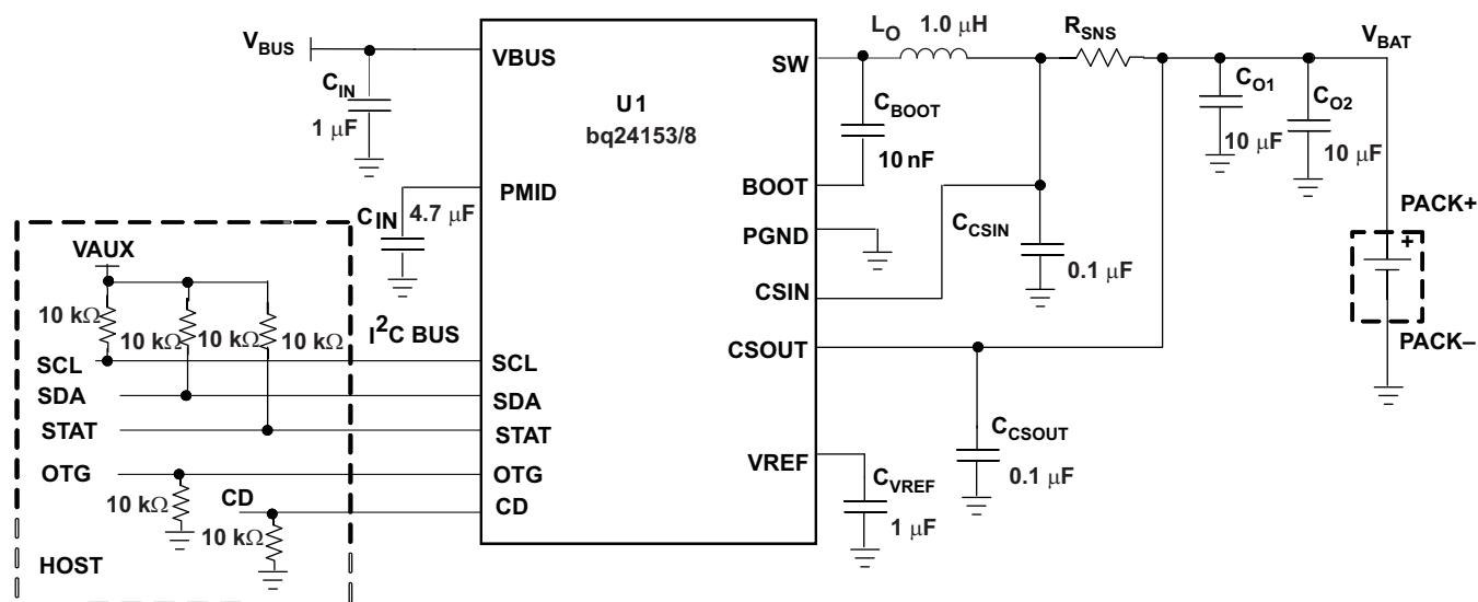
Figure 1. I²C Controlled 1-Cell USB Charger Application Circuit with USB OTG Support.
