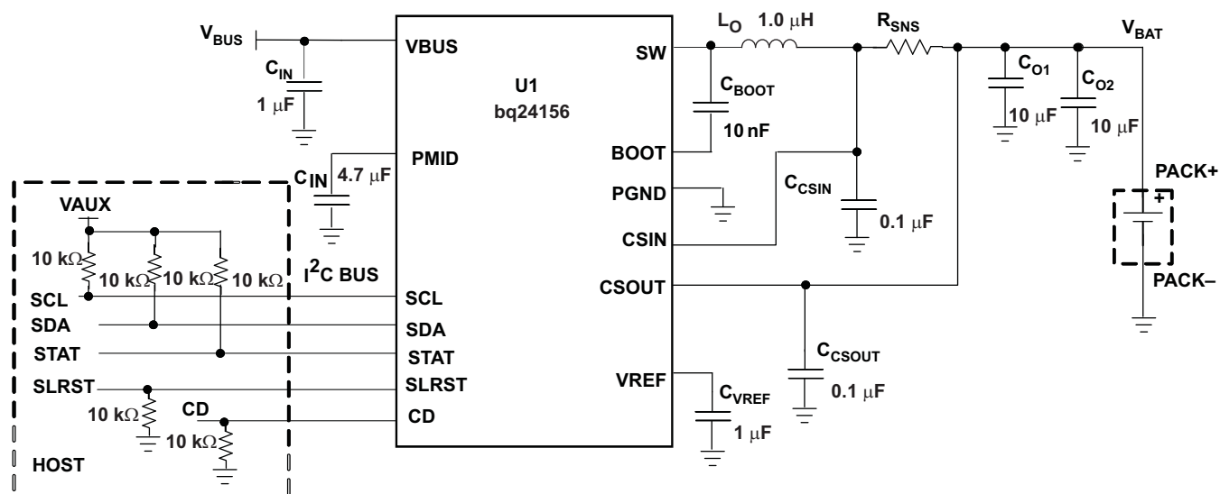
Figure 2. I²C Controlled 1-Cell Charger Application Circuit with External Safety Limit Register Control.
