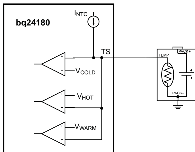
Figure 32. TS Circuit
