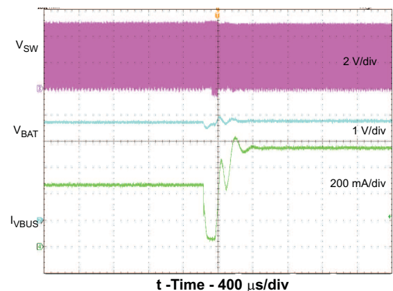
Figure 11. Input Current Limit Transition USB500 to 750mA
