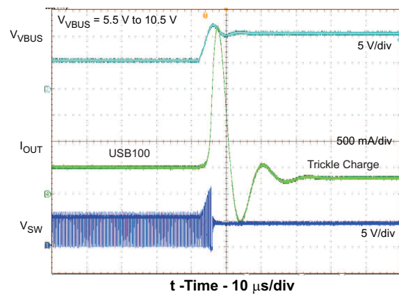
Figure 19. VINHIGH Response
