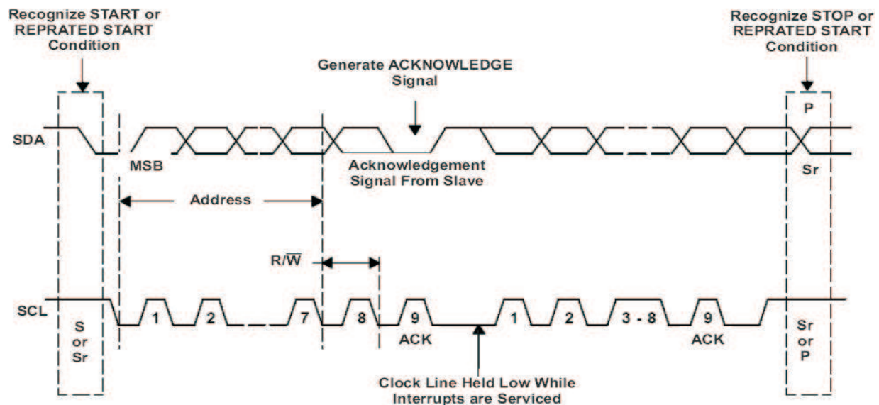
Figure 36. Bus Protocol
