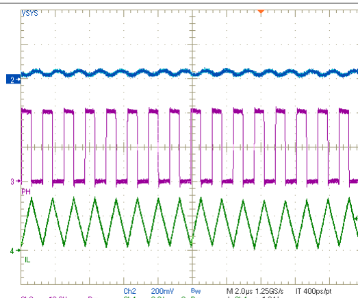
Figure 27. Current Disabled
