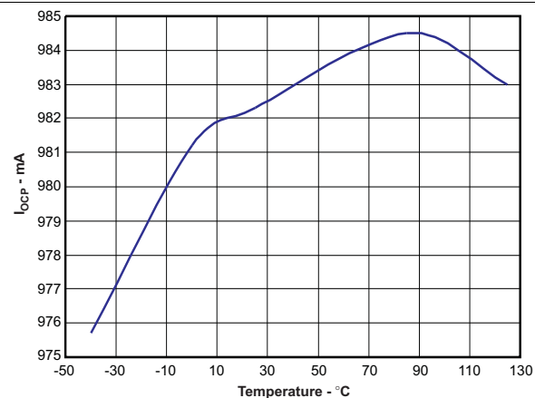
Figure 6. Input Overcurrent Protection vs Free-Air Temperature
