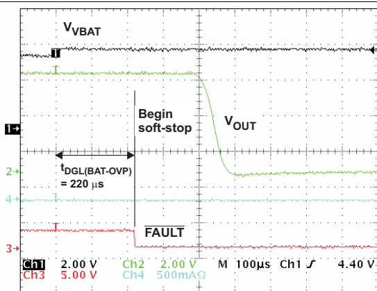
Figure 22. BAT-OVP, V_{BAT} Steps from 4.2\text{ V} to 4.4\text{ V} , Shows t_{DGL}(\text{BAT-OVP}) and Soft-Stop
