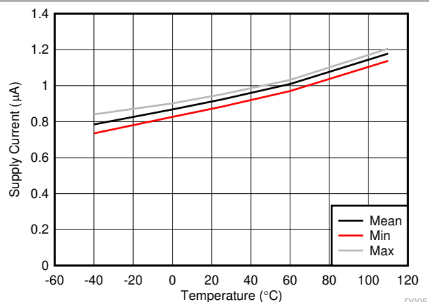
图 7-5. I_{DD} with Regulator Off
