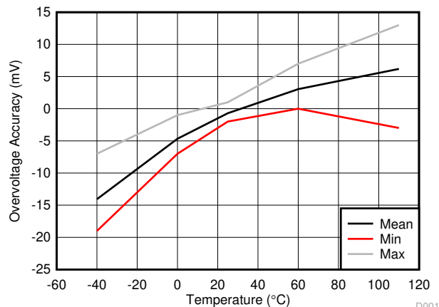
图 7-1. Overvoltage Threshold ( V_{OV} ) vs. Temperature
