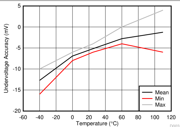
图 7-3. Undervoltage Accuracy
