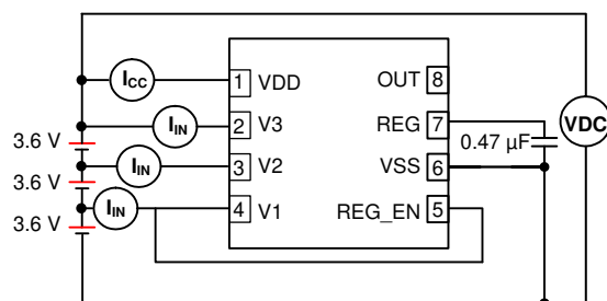
图 8-4. Configuration for Integrated Circuit Current Consumption Test
