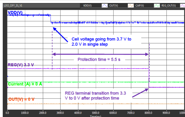
图 9-6. Undervoltage Detection to Turn Off the Regulator
