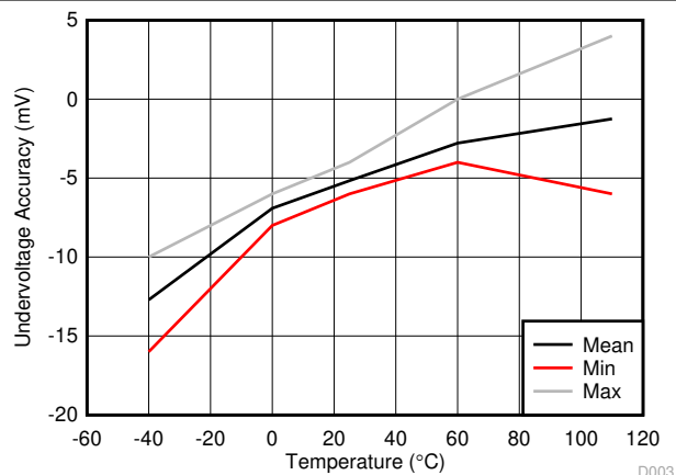
图 7-3. Undervoltage Accuracy
