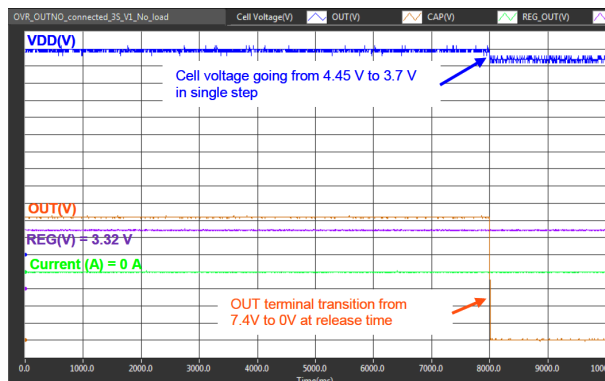
图 9-5. Overvoltage Protection Release
