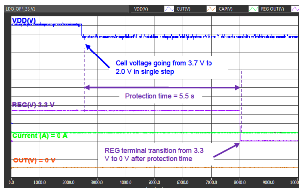
图 9-6. Undervoltage Detection to Turn Off the Regulator
