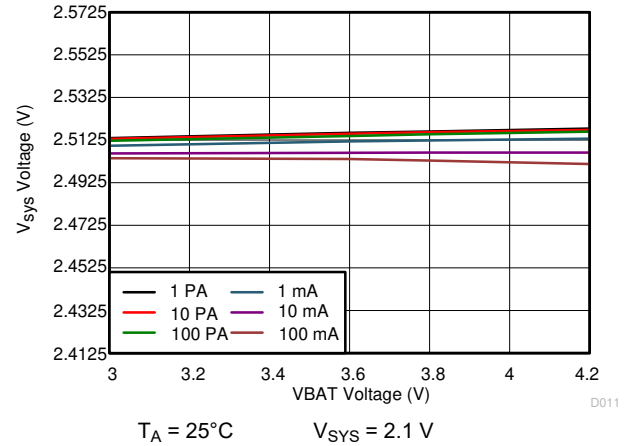
图 10-23. 2.1 V_{\text{SYS}} Line Regulation
