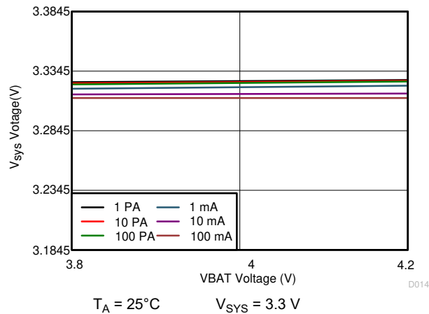
图 10-24. 3.3 V_{\text{SYS}} Line Regulation
