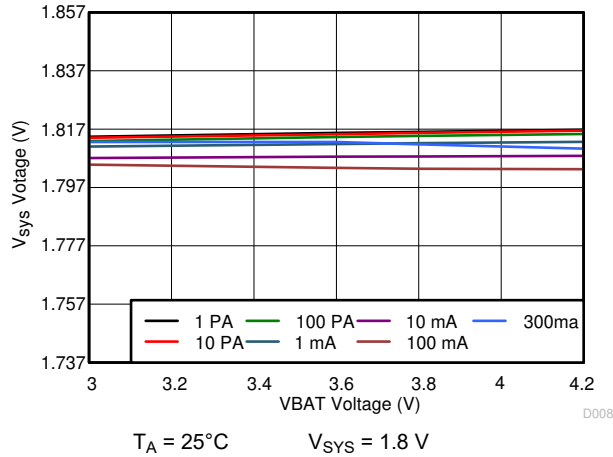
图 10-22. 1.8 V_{\text{SYS}} Line Regulation
