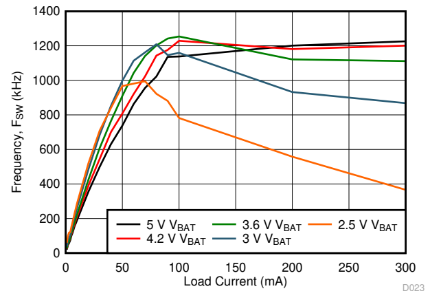
图 10-25. 1.8 V_{\text{SYS}} Switching Frequency vs Load Current
