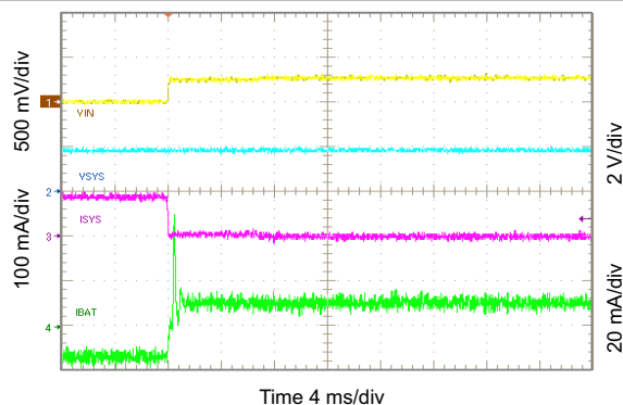
图 10-7. Exiting Battery Supplement Mode
