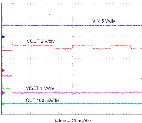
图 7. DPM-Adaptor Current Limits
