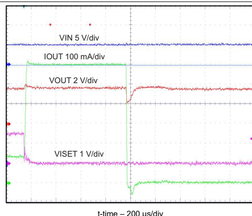
图 8. Hot Plug Source with No Battery - Battery Detection
