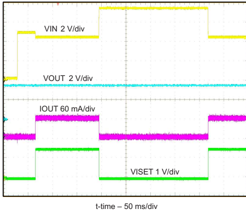
图 5. OVP from Normal Power-Up Operation
