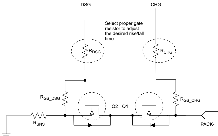
图 10-1. Select Proper Gate Resistor for FET Rise and Fall Time
