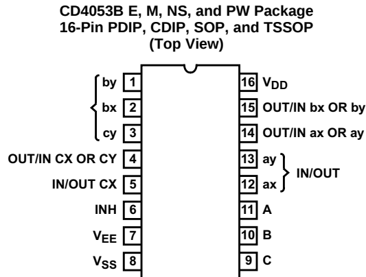
Pin Functions CD4051B
