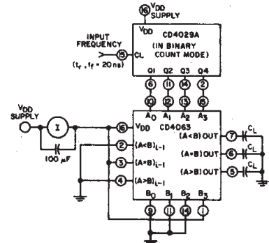
Fig. 12 - Dynamic power dissipation test circuit.
