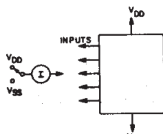
Fig. 11 - Input current test circuit.
