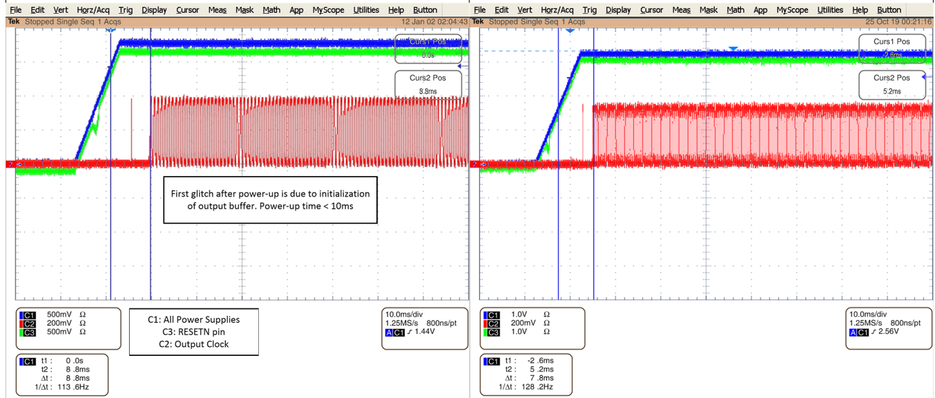
Figure 5. All Power Supply = 1.8 V, VDD Ramp Time = 1 ms
