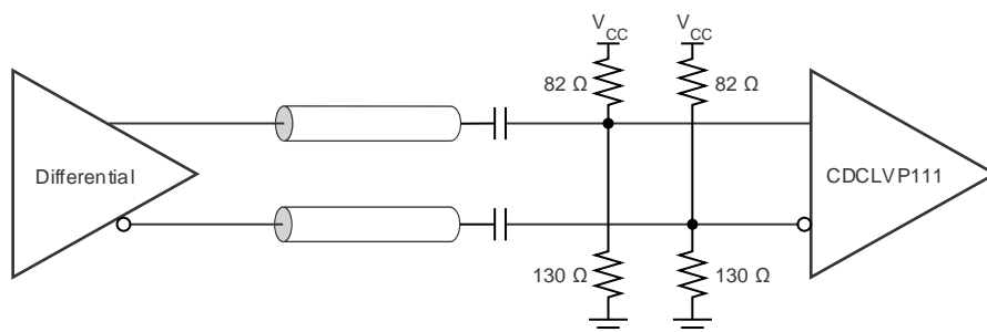
Figure 15. AC-Coupled Differential Inputs to CDCLVP111 ( V_{CC} = 3.3 V)
