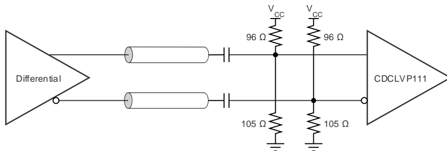
Figure 14. AC-Coupled Differential Inputs to CDCLVP111 ( V_{CC} = 2.5 V)
