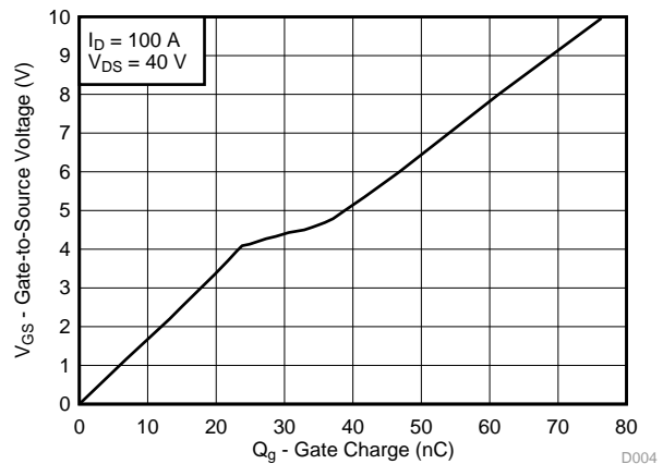
栅极电荷
