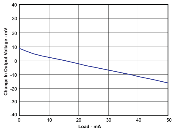
图 11. LDO Load Response
