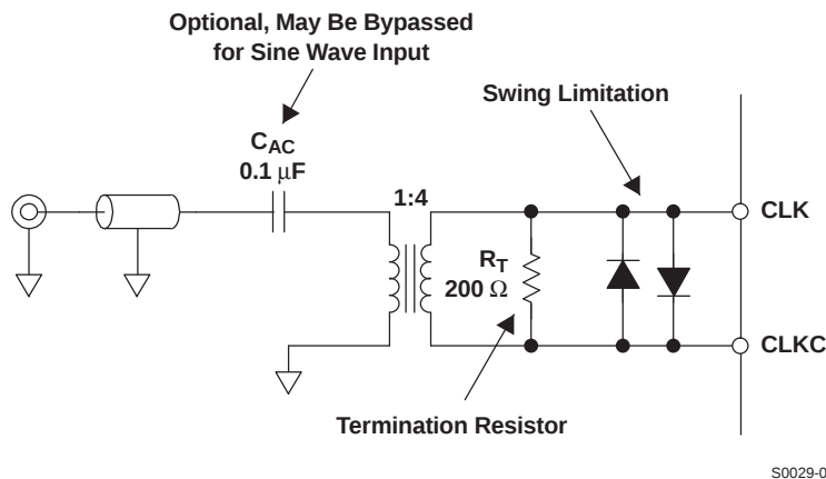
Figure 65. Clock Input Configuration Using 50- \Omega Cable Input
